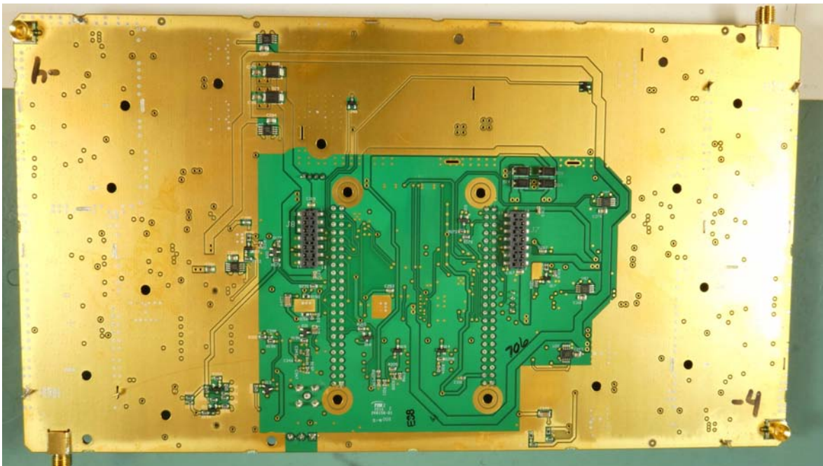
Control and LNA PCBA 3-26063-4 Rear view
