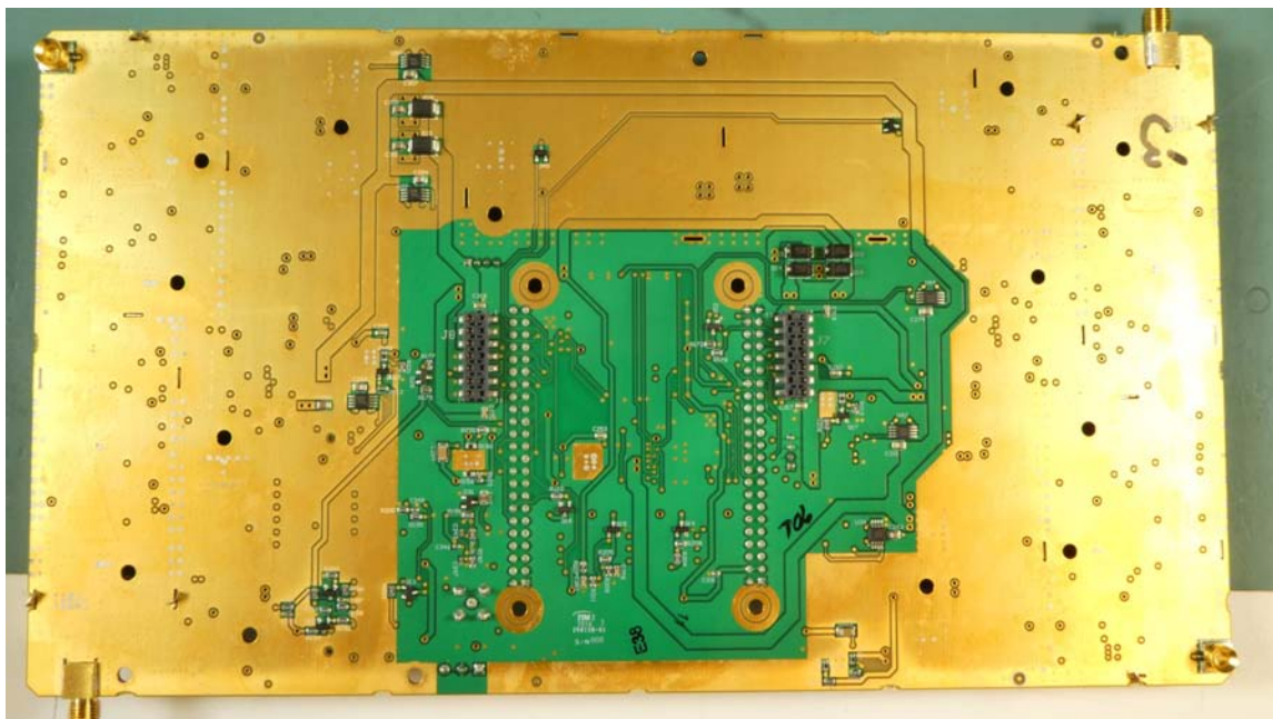
Control and LNA PCBA 3-26063-3 Rear view
