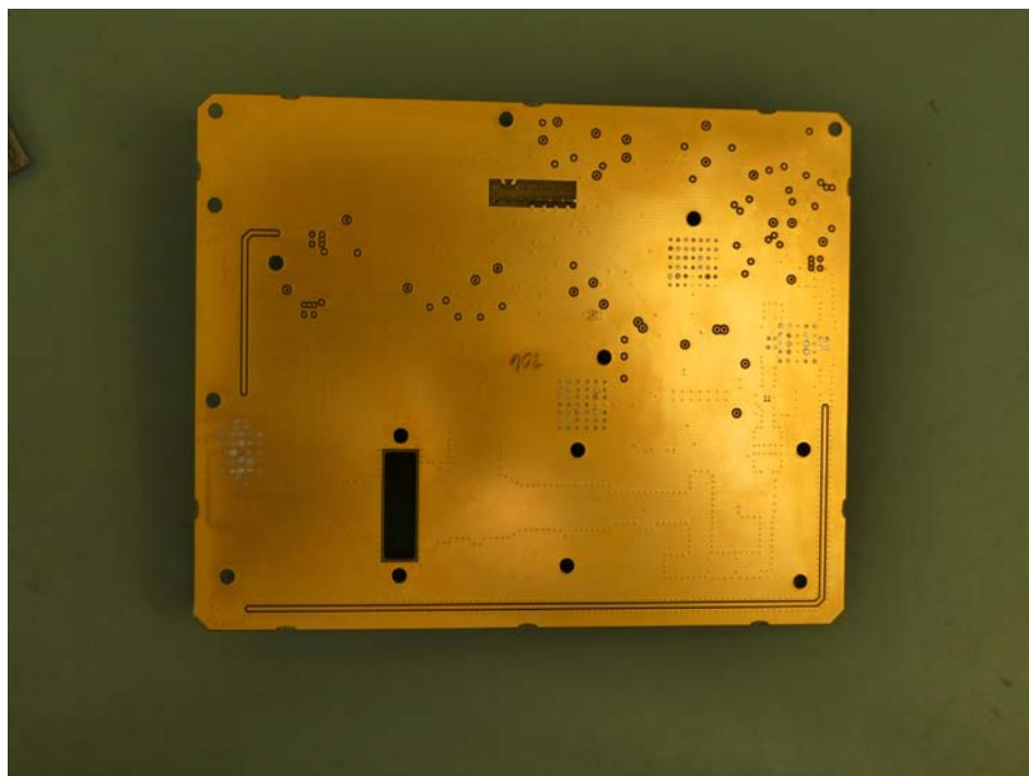
Power Amplifier PCBA 3-26070-1 Rear view
