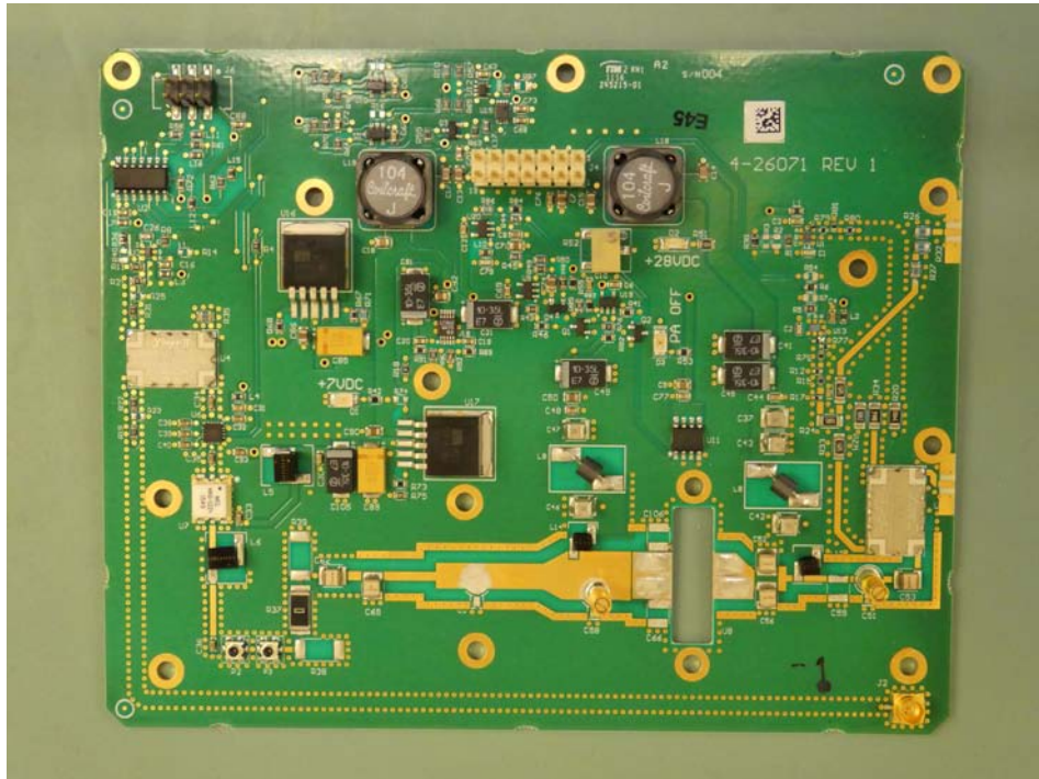
Power Amplifier PCBA 3-26070-1 Front view
