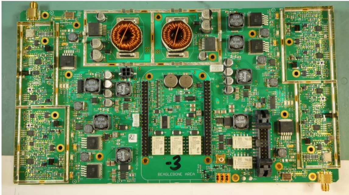
Control and LNA PCBA 3-26063-3 Front view
