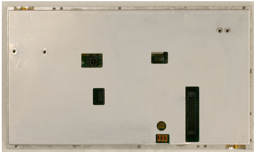
Control and LNA Assembly 3-26062-5 Top view.
