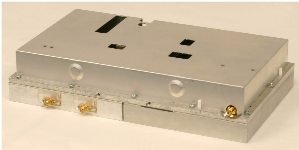
Class B SB Module 3-26076-1S Rear-side view.
