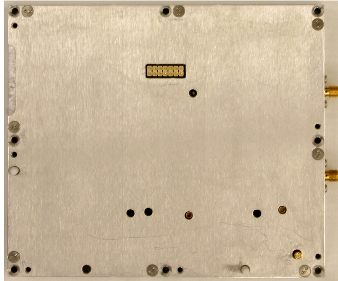
Uplink Power Amplifier Assembly 3-26072-1 Top view.
