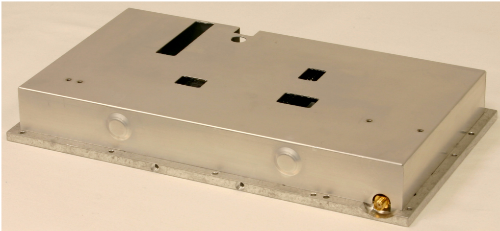
Control and LNA Assembly 3-26062-5 Rear-side view.
