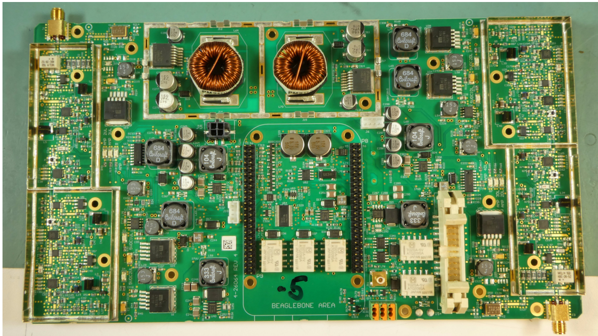
Control and LNA PCBA 3-26063-5 Front view
