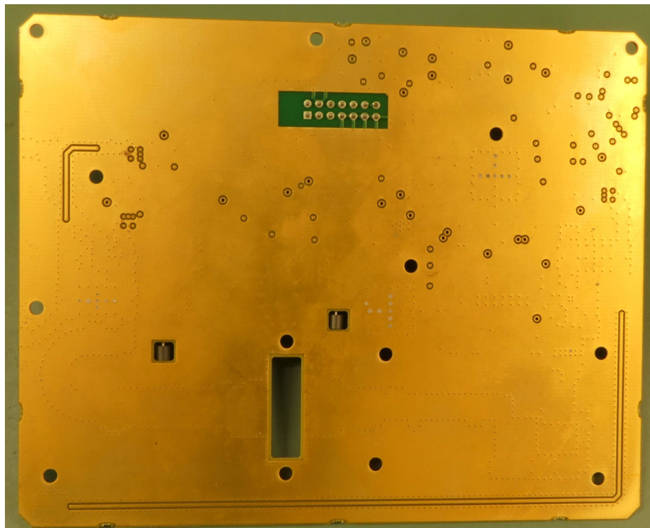
Power Amplifier PCBA 3-26073 Rear view
