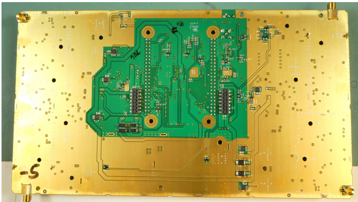
Control and LNA PCBA 3-26063-5 Rear view
