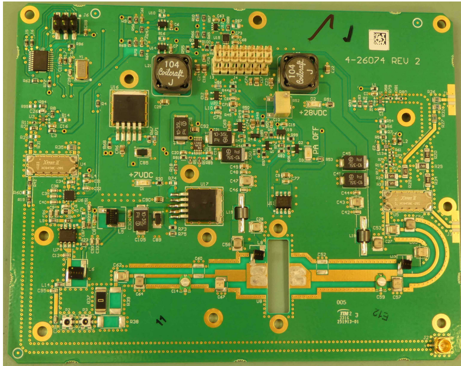
Power Amplifier PCBA 3-26073 Front view
