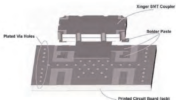
Figure 4: Mounting Features Example
