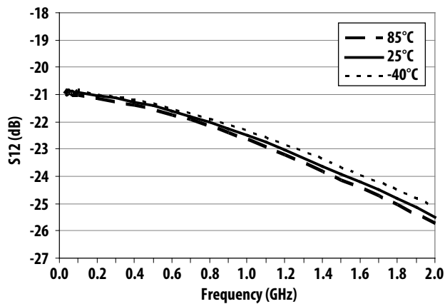
Figure 12. S12 over Frequency and Temperature
