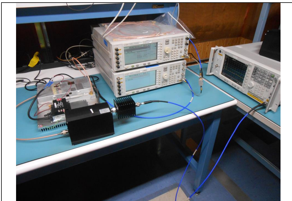
RF Conducted #1
