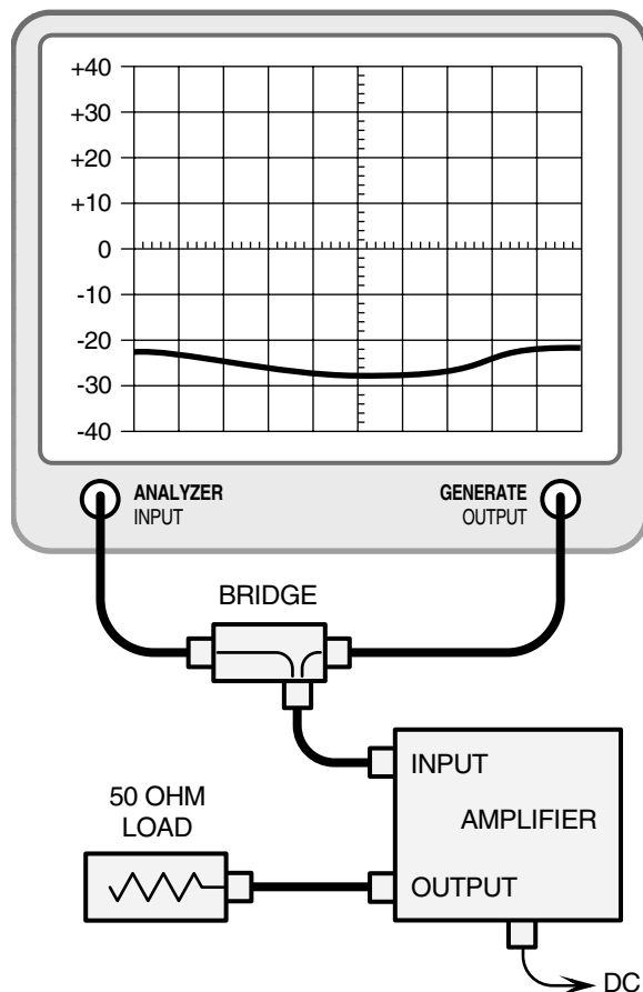
Figure 7: Measuring output return loss.
