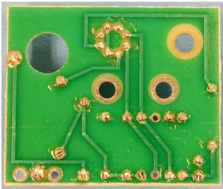
3-10742 Bias Circuit Board Assembly
