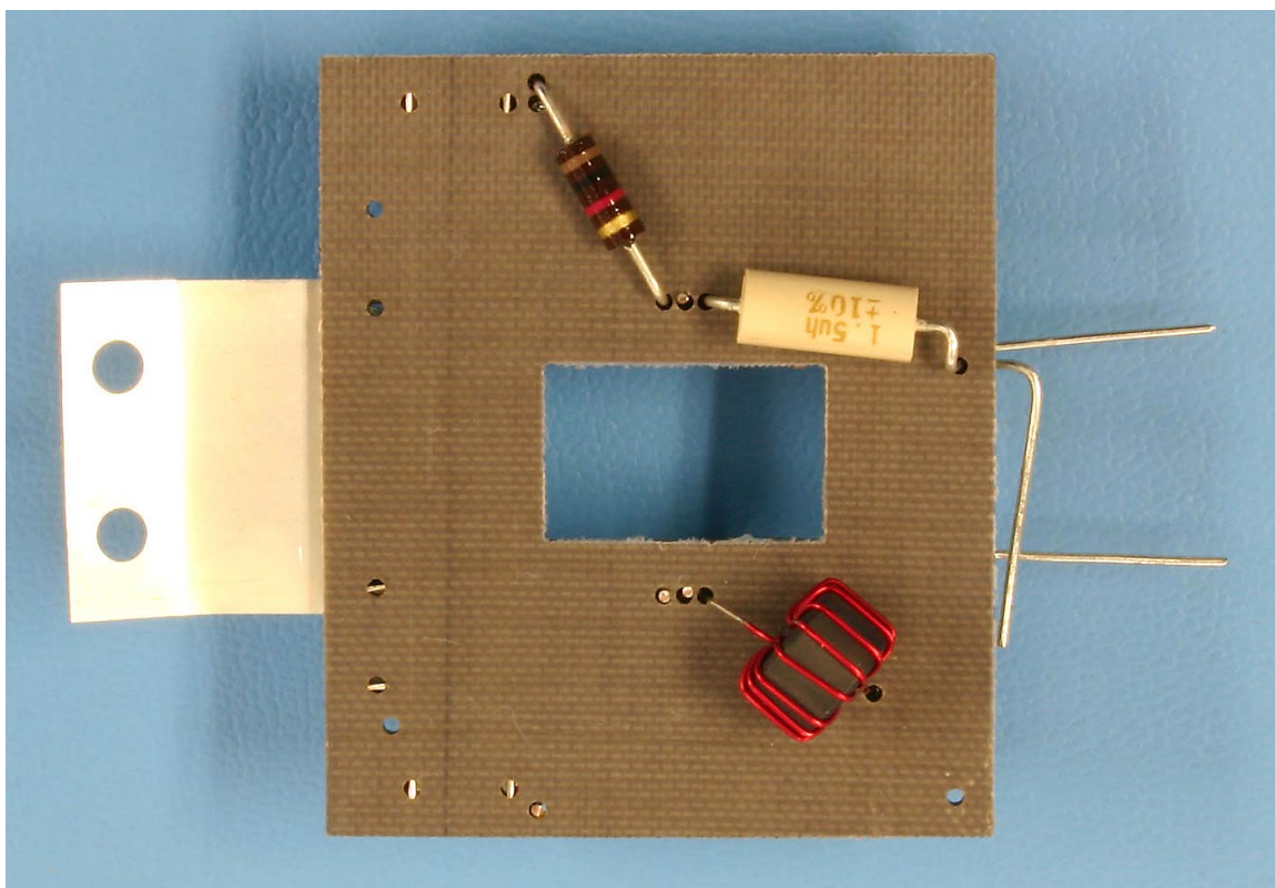
3-8087 RF Circuit Board Assembly
