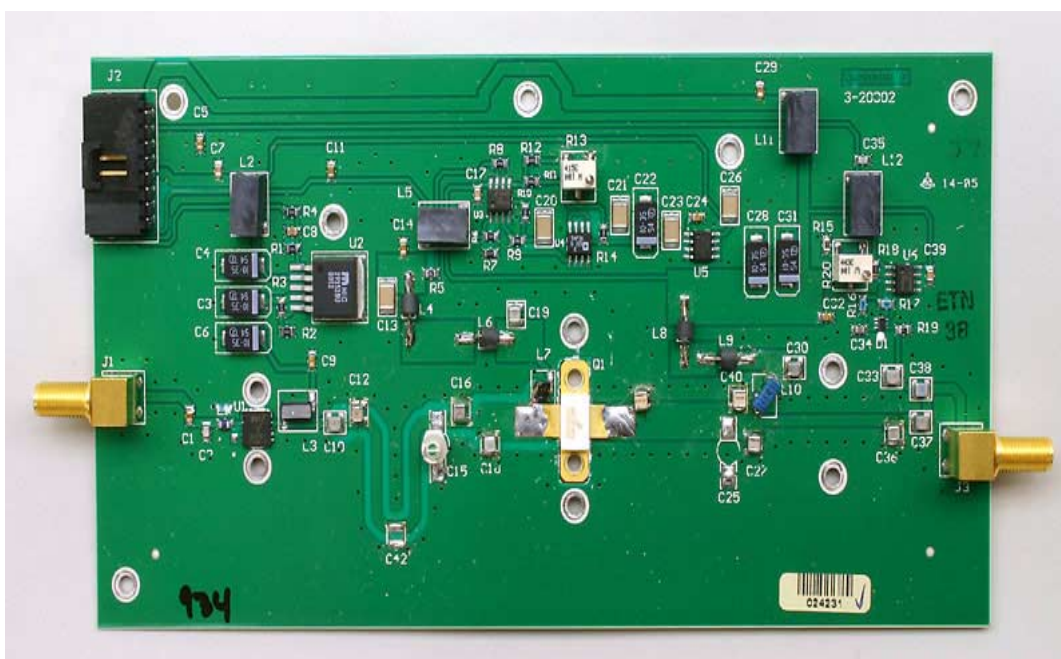
3-20807 Power Amplifier Assembly Front PCB View
