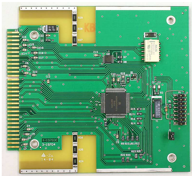
3-19832 Control Card Front PCB View
