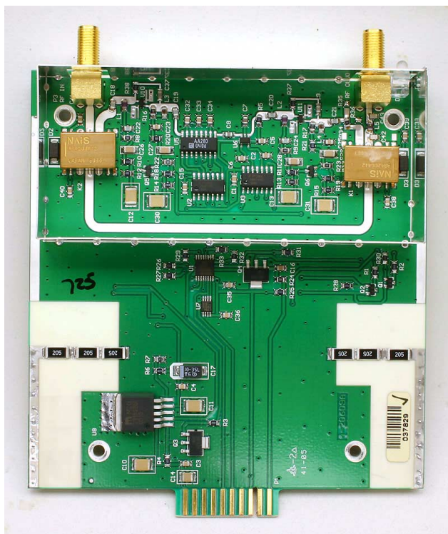
3-19935 Low-Level Amplifier Assembly Front PCB View
