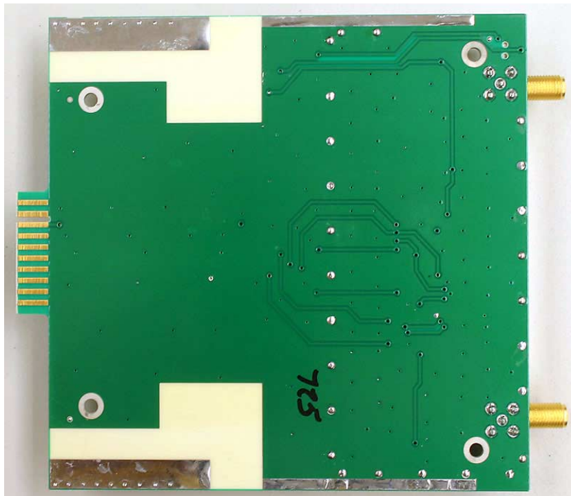
3-20208 Attenuator Card Back PCB View
