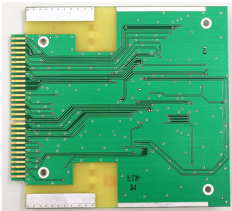
3-19832 Control Card Back PCB View
