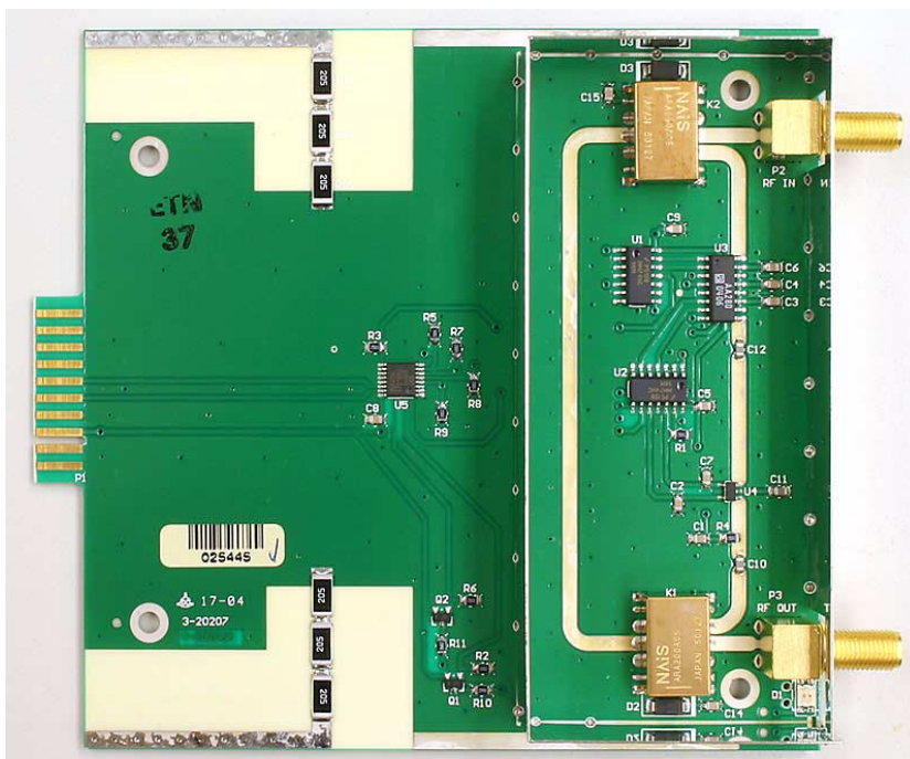
3-20208 Attenuator Card Front PCB View
