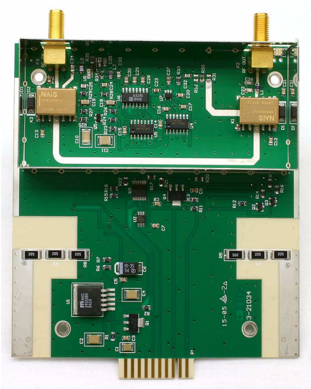
3-21035 Half-Gain Low-Level Amplifier Assembly Front PCB View
