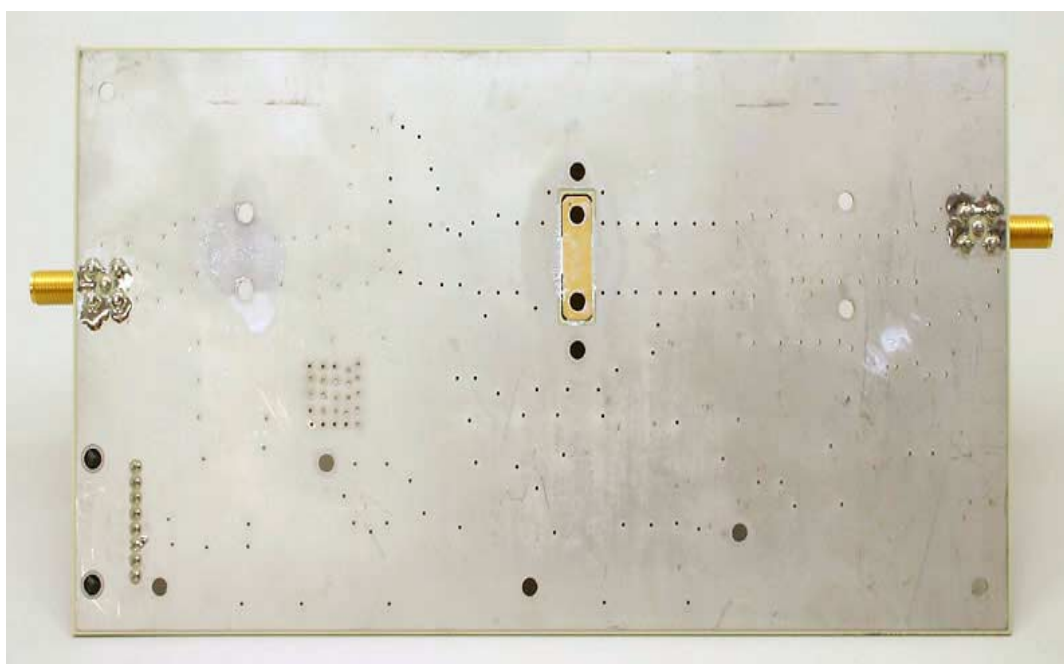
3-20807 Power Amplifier Assembly Back PCB View
