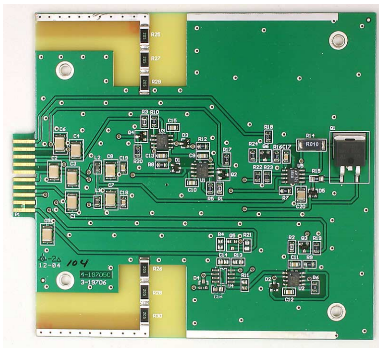
3-19833 Power Distribution Card Front PCB View
