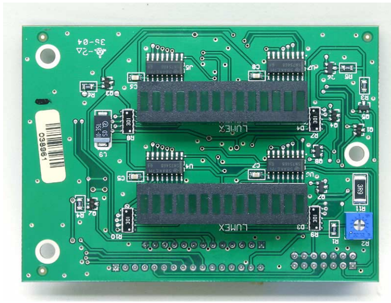
3-19708 Display Circuit Board Front PCB View
