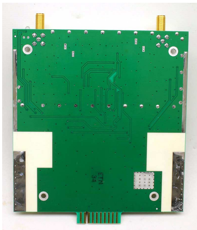
3-19935 Low-Level Amplifier Assembly Back PCB View
