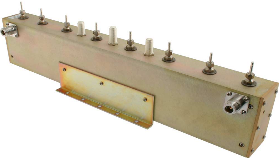
3-21111 Filter Assembly
