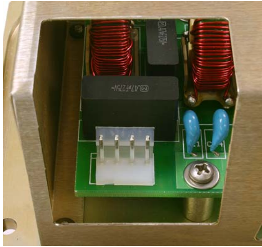
AC Power Supply 3-23912 AC Input close-up.
