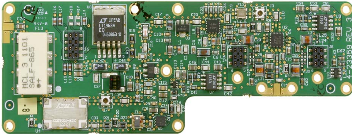
Channel Module Upconverter board 3-23357-8 top view.
