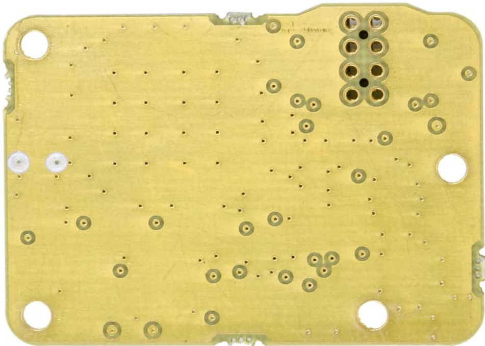
Channel Module Oscillator board 3-23351-1 bottom view.
