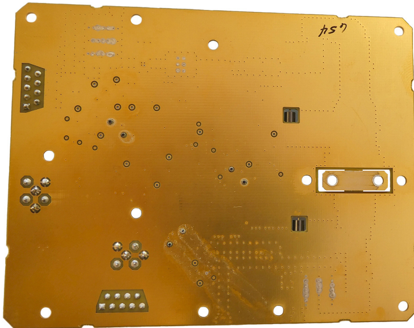
Power Amplifier Board 3-23366 back view. (used in subassembly 3-23912)
