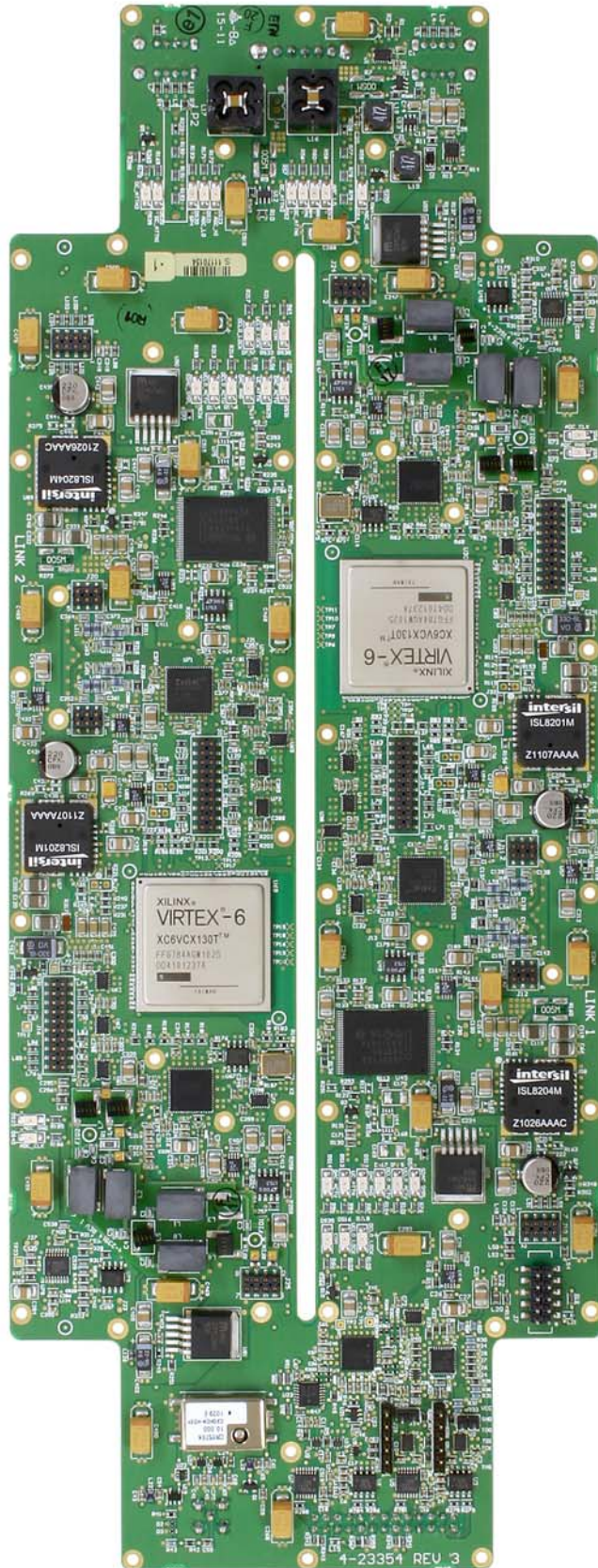
Channel Module Digital board 3-23353-1 top view.
