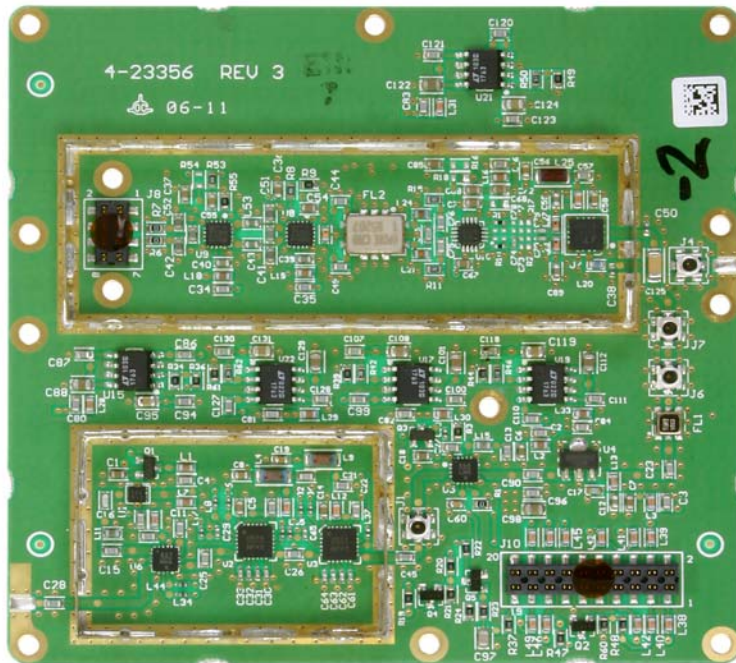
Channel Module Downconverter board 3-23355-2 top view.
