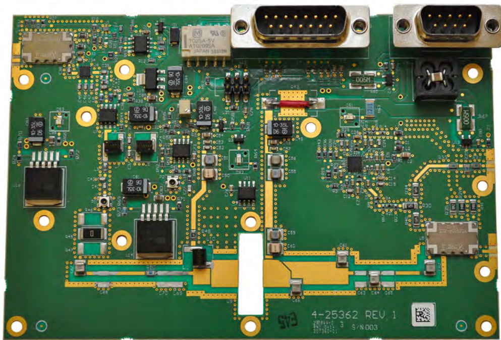
Power Amplifier Board 3-25631 front view
