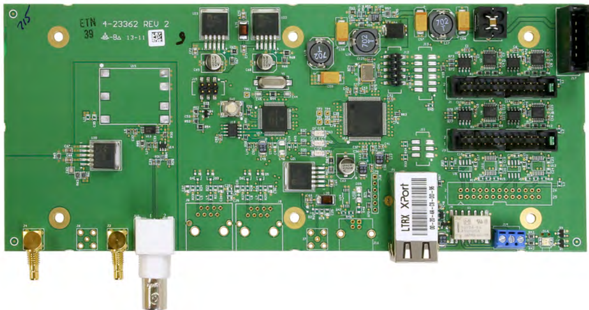
Controller Board 3-23361-1 front view
