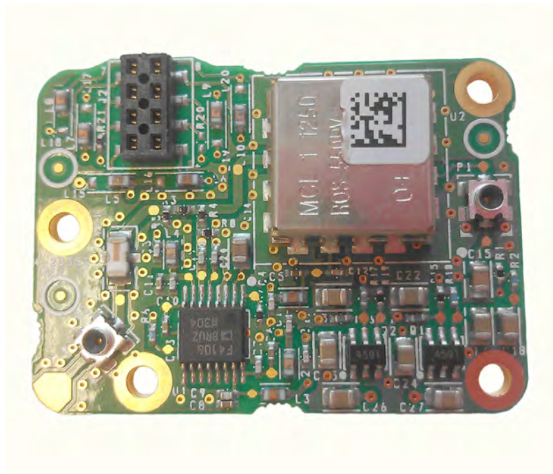
Local Oscillator Board 3-25115 (1 through 4) front view
