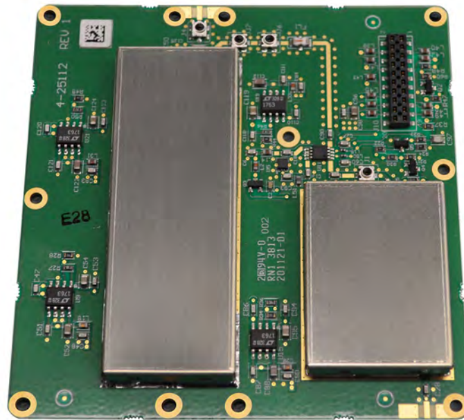
Downconverter Board 3-25111 front view
