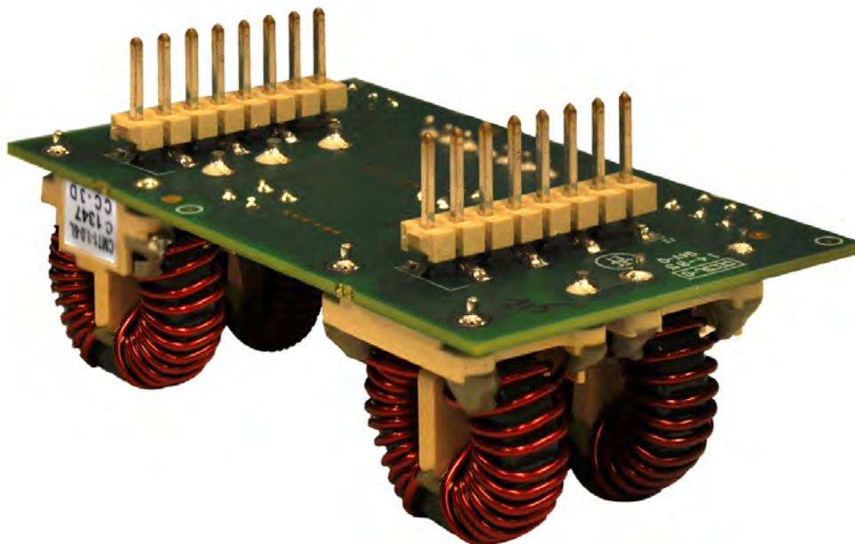
Power Supply Daughter Board 3-25363 side view
