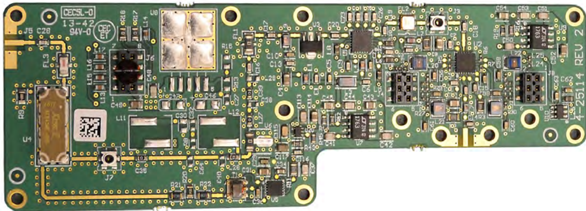
Upconverter Board 3-25113-3 front view
