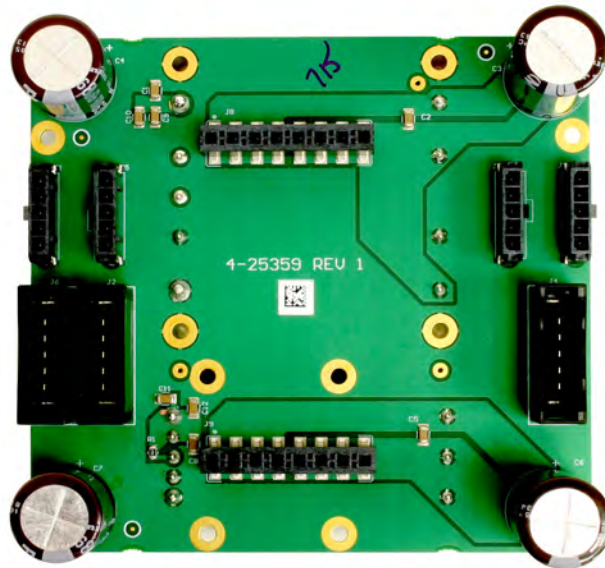
Power Supply Mother Board 3-25358 front view
