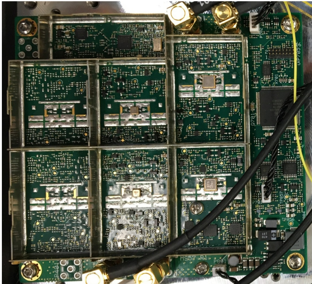
KS 57.52 – Front VGA
