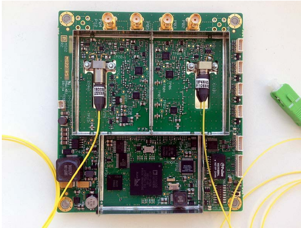
KS22.1 – Front FOR Fiber optic board
