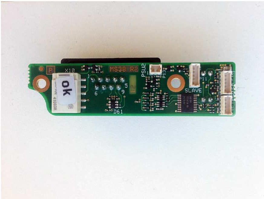
KS38.2 – Back – AIO Alarm board
