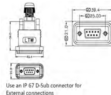
Figure 58 External Alarm Connector
