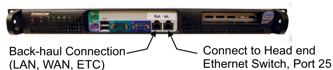
Figure 28 BGW Installation, Ethernet Connections
