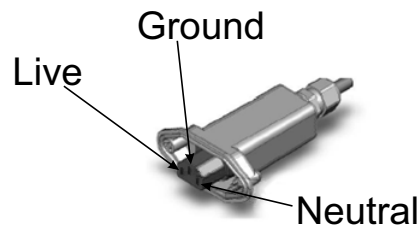
Figure 57 Weatherproof AC Input Connector
