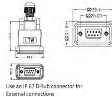
Figure 48 External Alarm Connector
