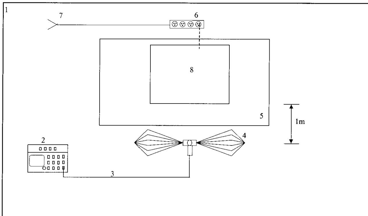
Figure 2. Test Configuration, Frequency Identification of Radiated Emissions
