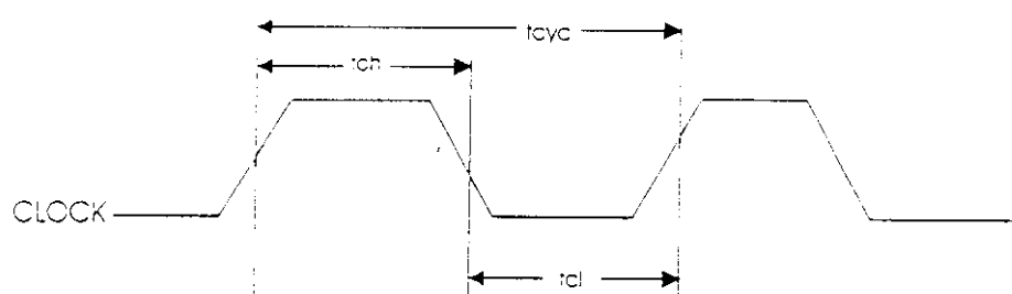
Clock Timing
