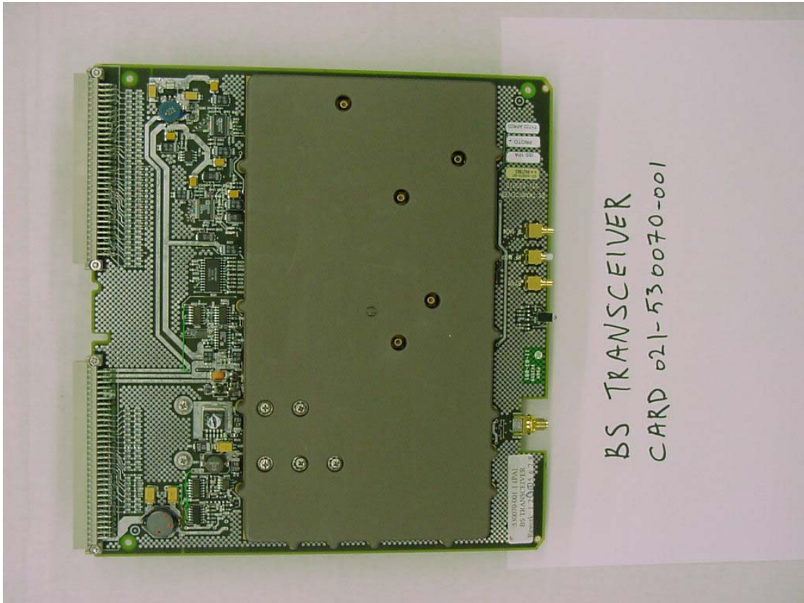
SBS Transceiver With Cover
