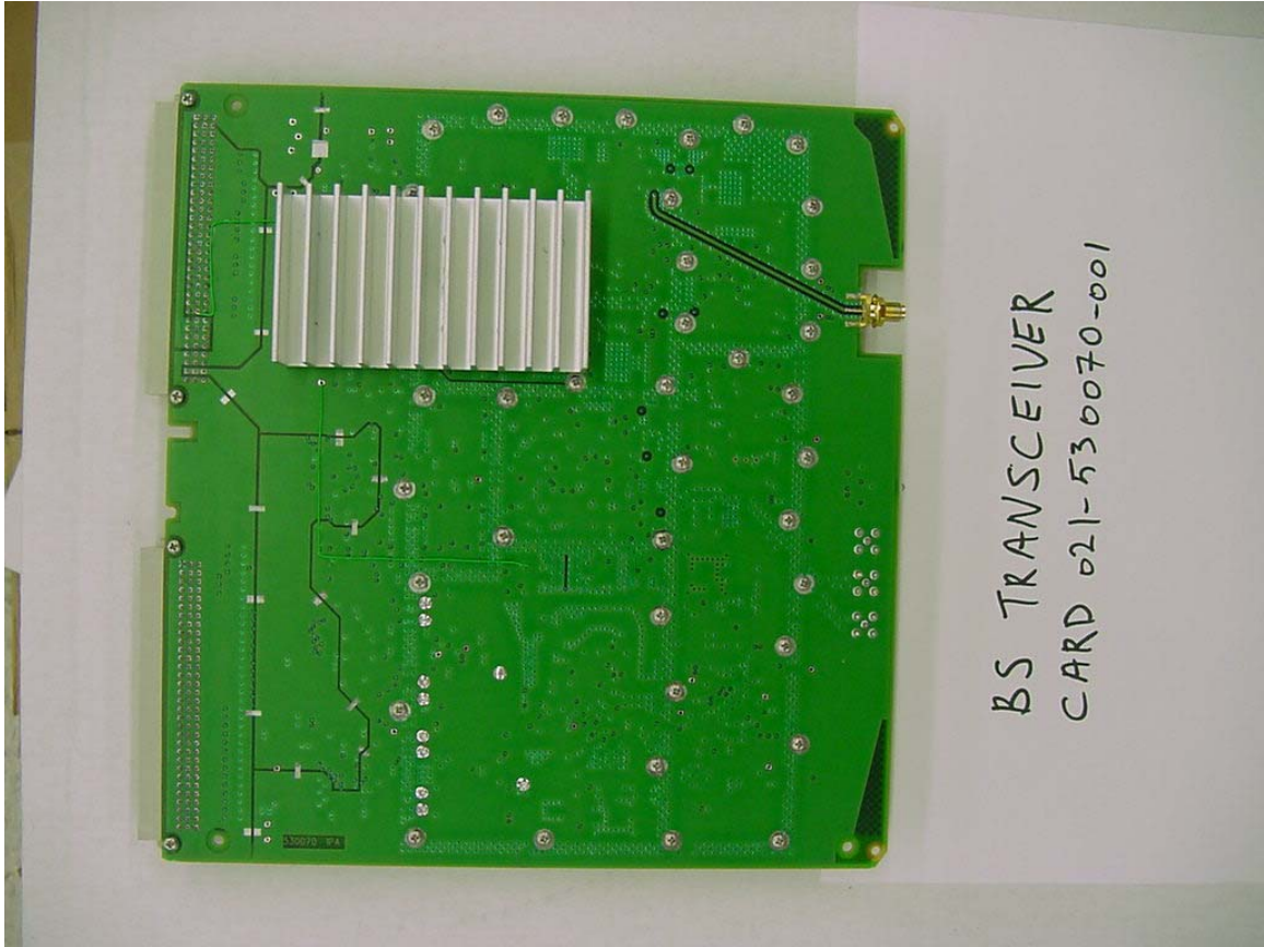
SBS Backplane
