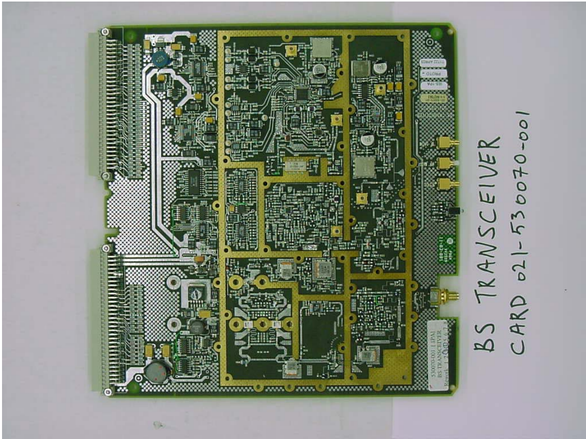
SBS Transceiver No Cover
