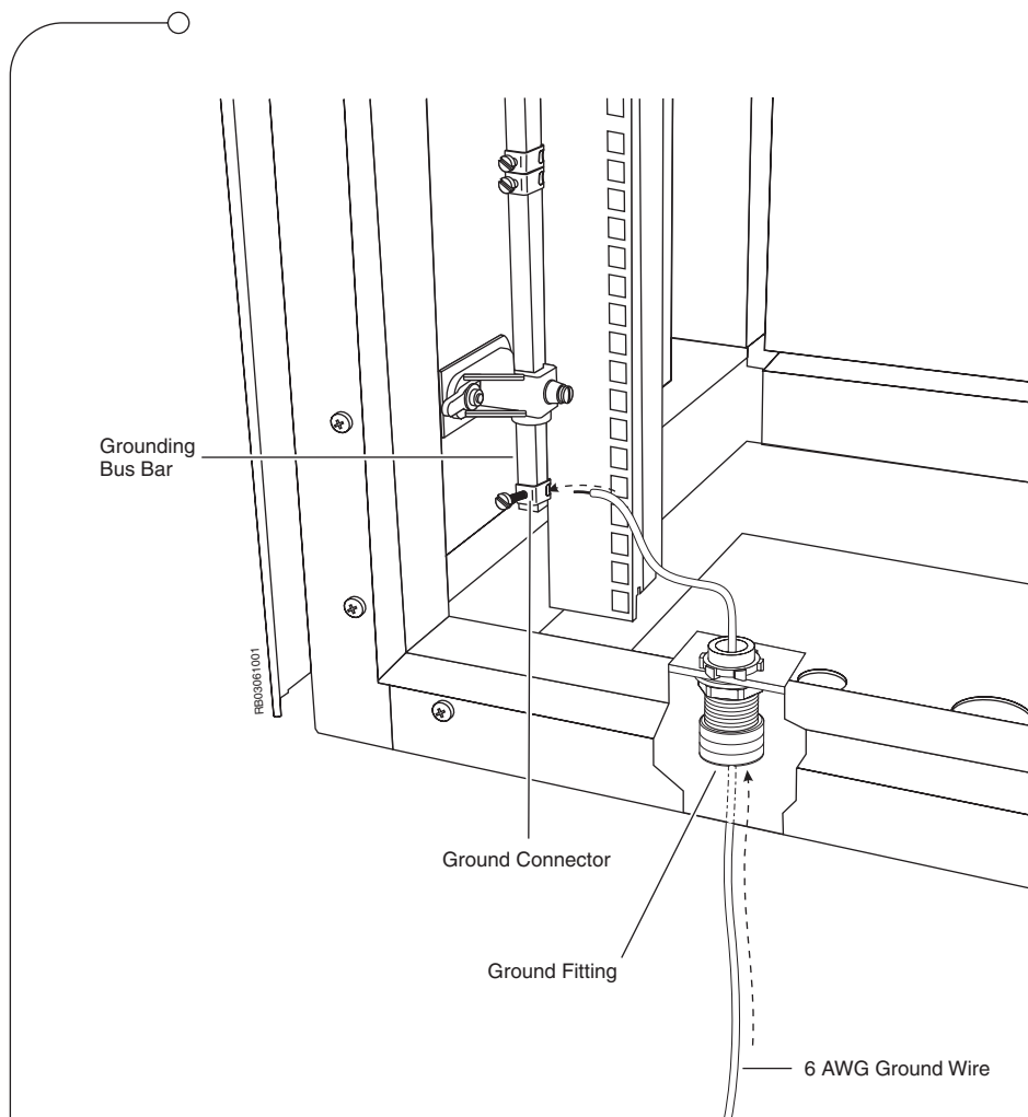
Figure 3.12 Ground Connection
