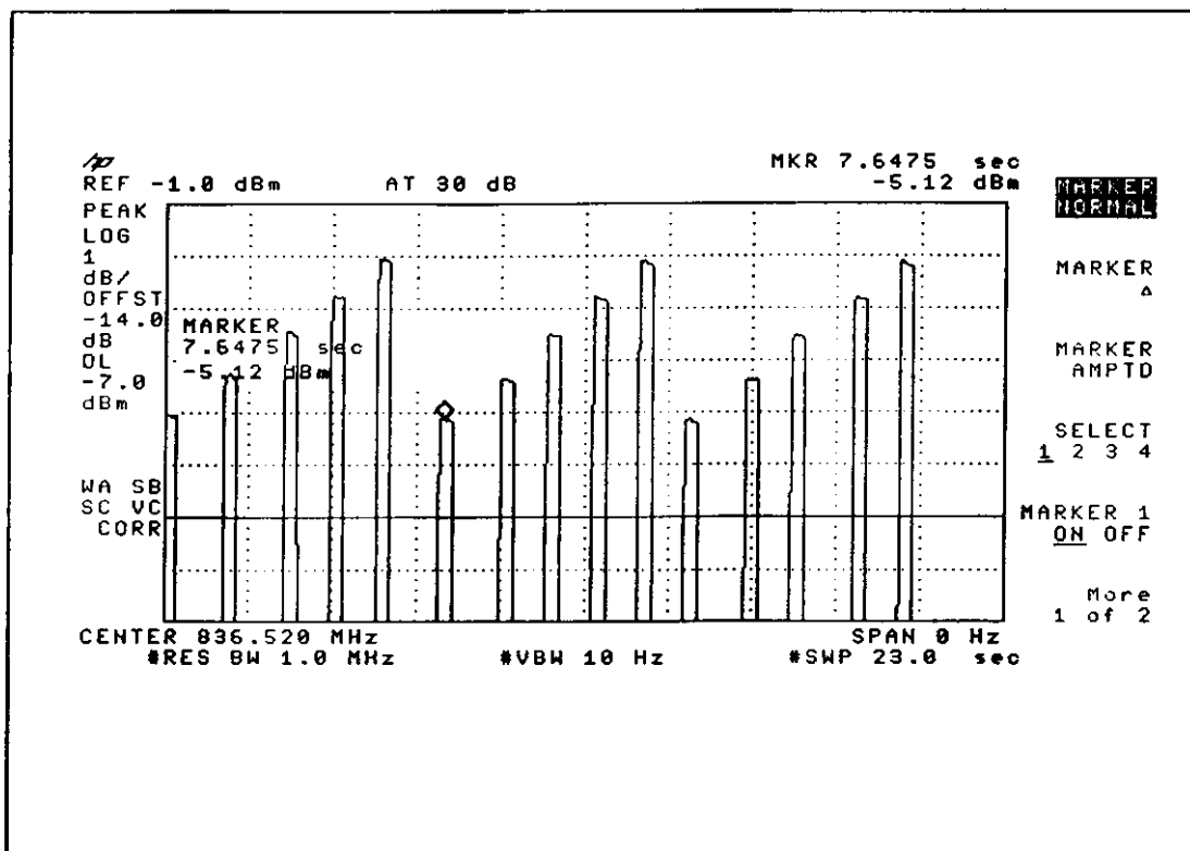
Figure 2.4.3.1 Test result printing for Test 2 (#1)
