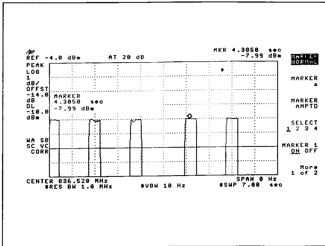
Figure 2.4.3.1 Test result printing for Test 1 (#1)
