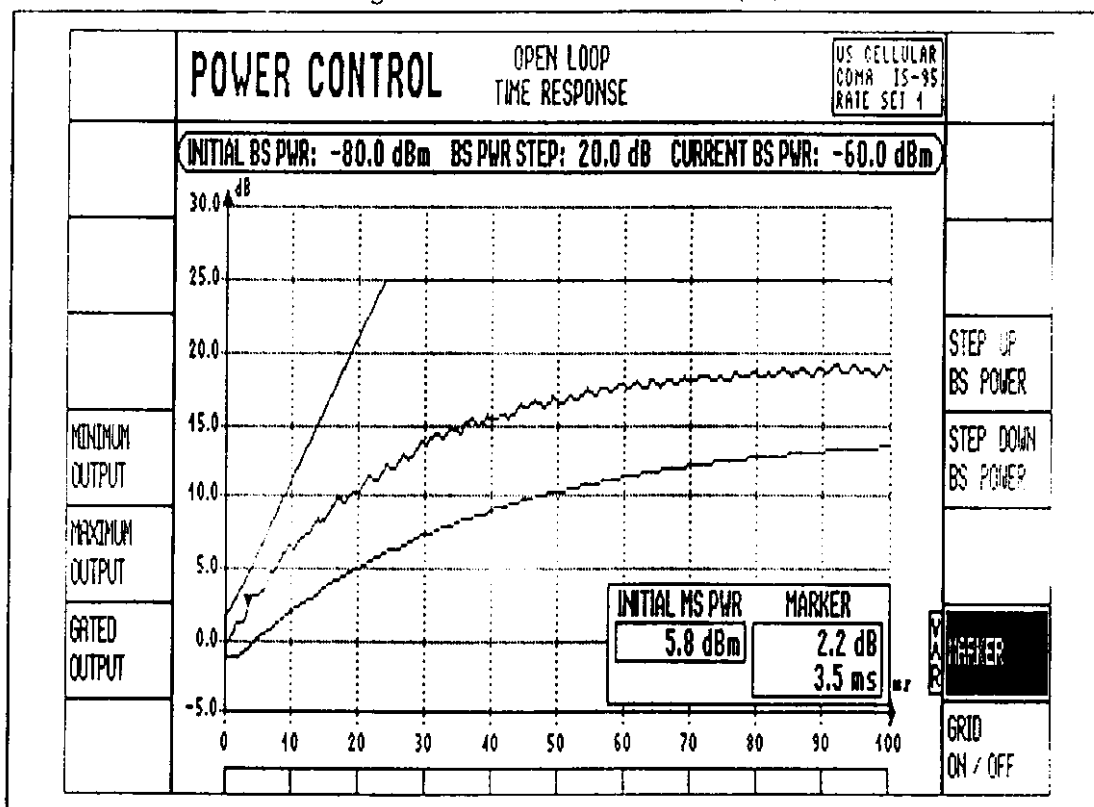
Figure 2.4.2.4 Test result for Test 4 (#1)
