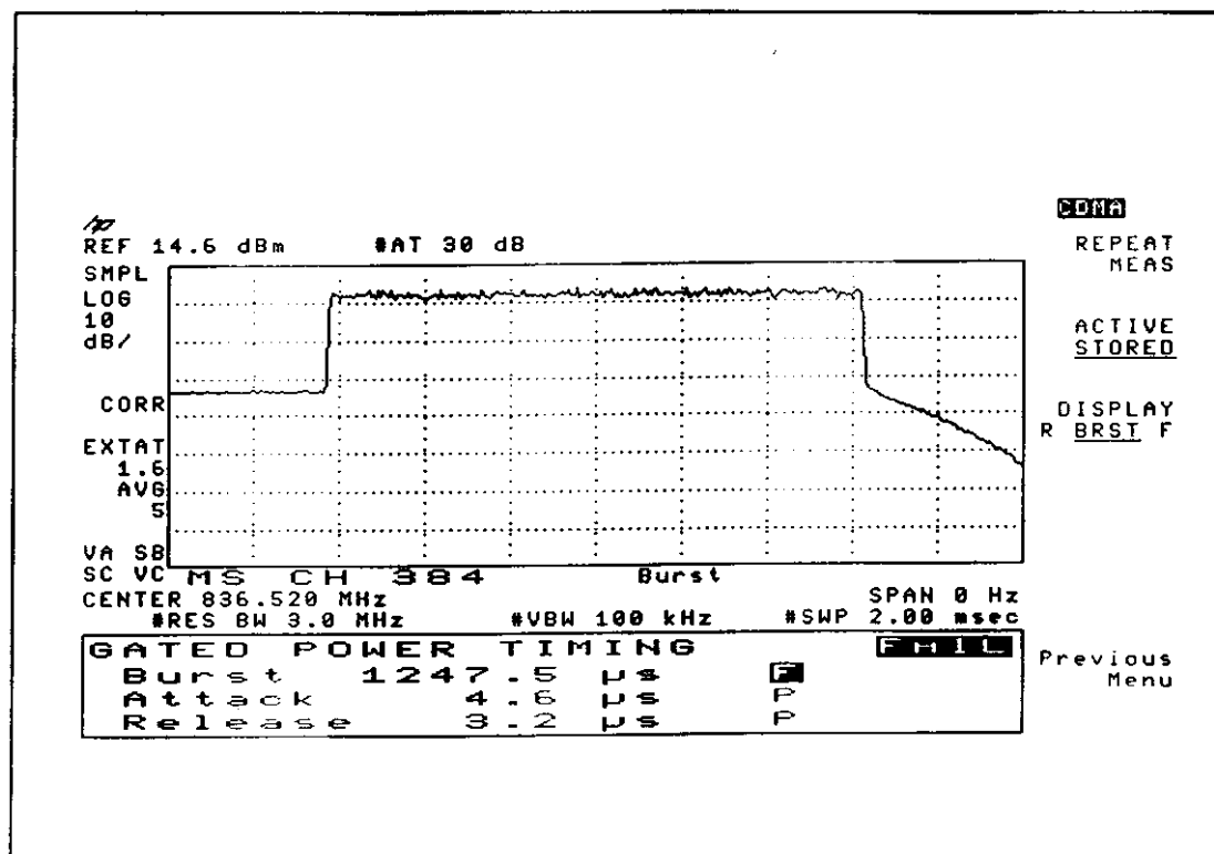
Figure 2.4.7.1 Test result printing for Gated Output Power (#1)
