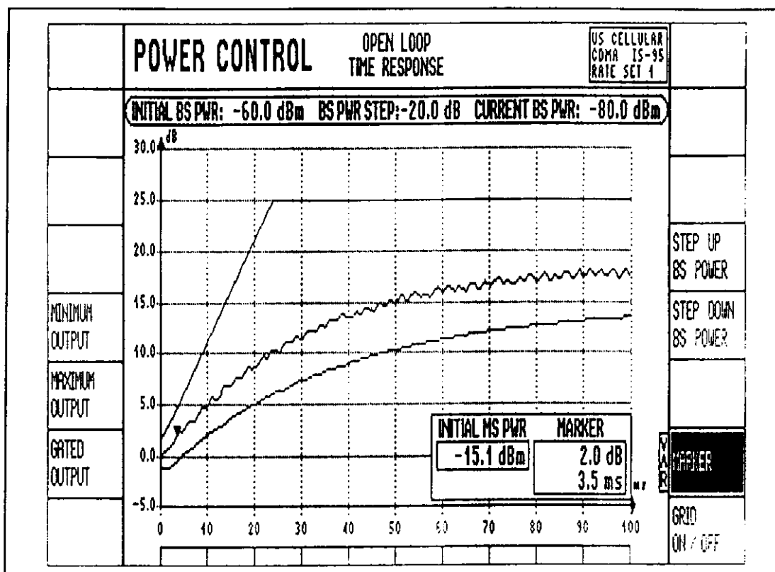
Figure 2.4.2.3 Test result for Test 3 (#1)
