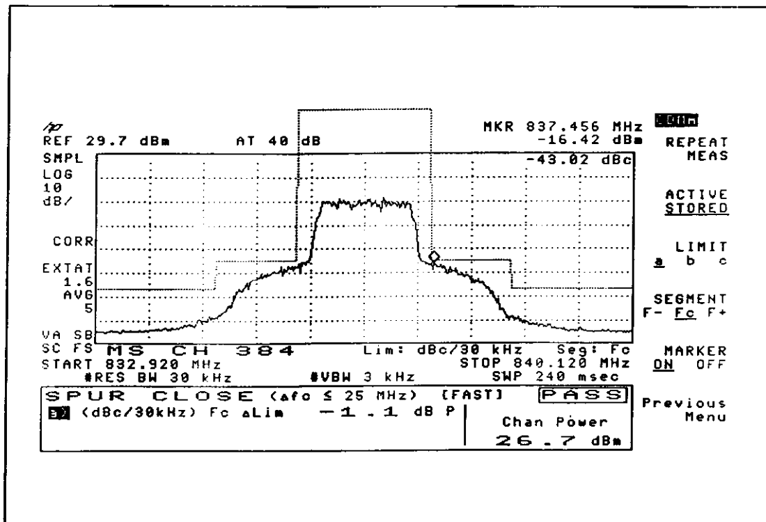
Figure 2.5.1.2 Test result printing for Spurious Emission When Transmitting. (#2)
