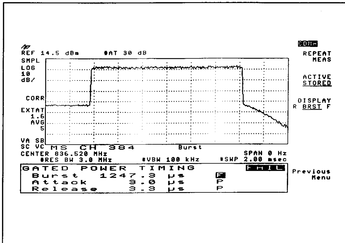
Figure 2.4.7. Test result printing for Gated Output Power (#2)
