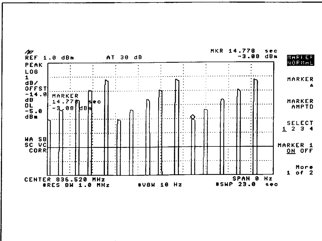
Figure 2.4.3.2 Test result printing for Test 2 (#1)
