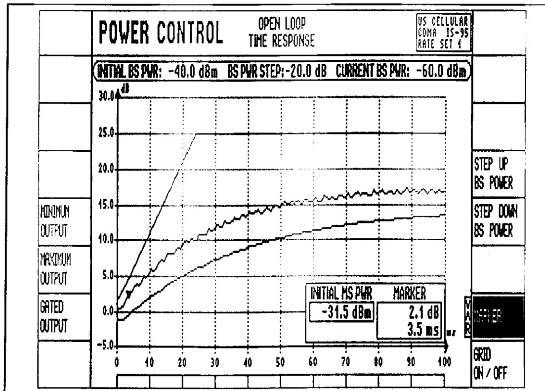
Figure 2.4.2.6 Test result for Test 2 (#2)
