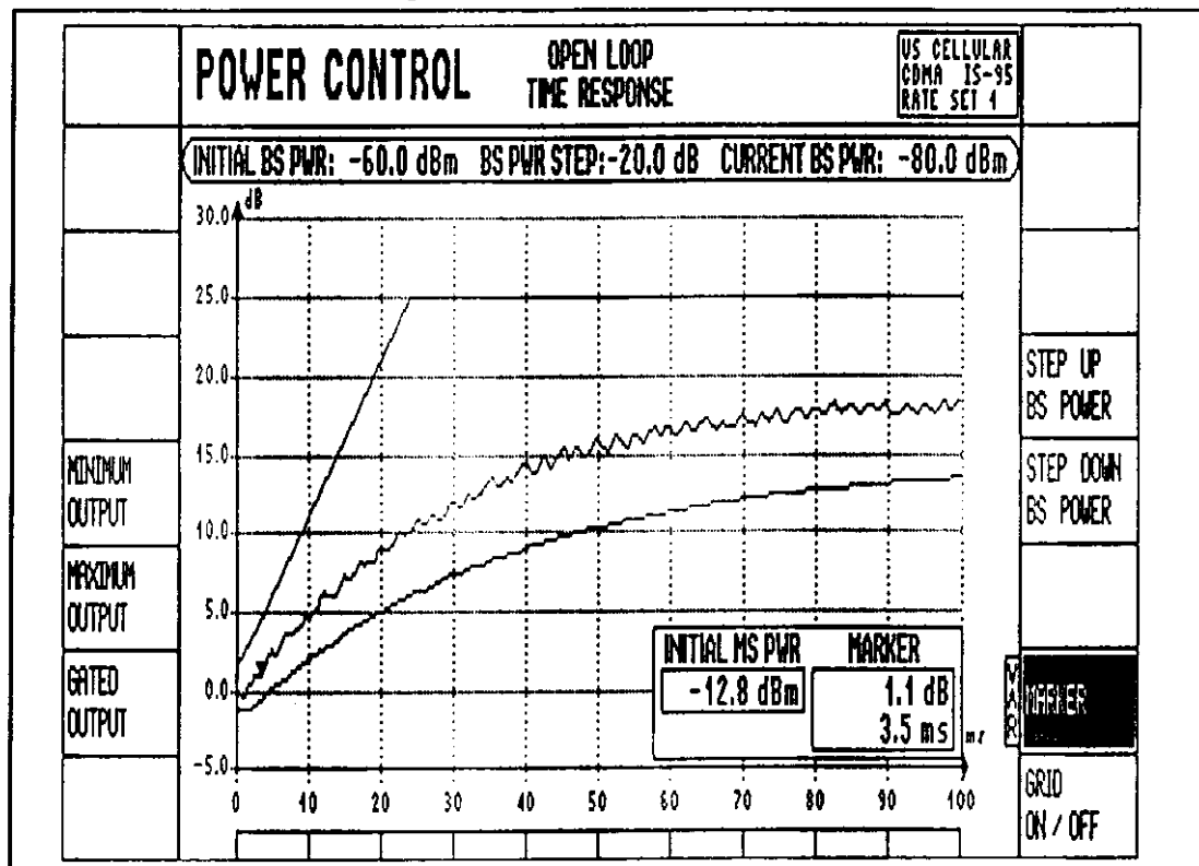
Figure 2.4.2.7 Test result for Test 3 (#2)
