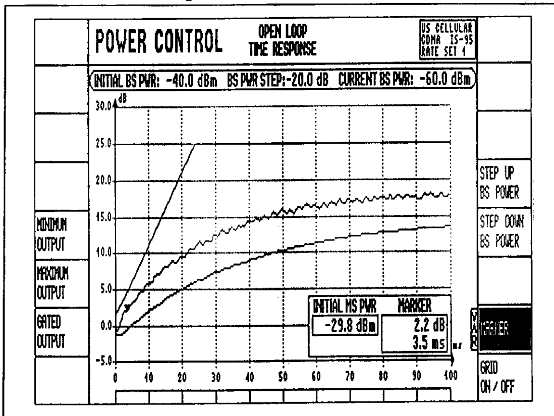
Figure 2.4.2.2 Test result for Test 2 (#1)
