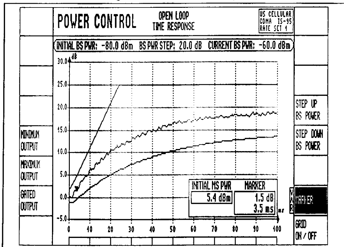
Figure 2.4.2.8 Test result for Test 4 (#2)
