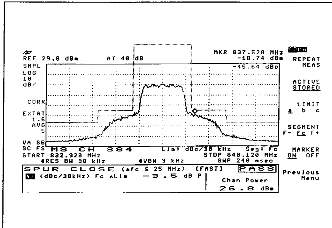
Figure 2.5.1.1 Test result printing for Spurious Emission When Transmitting. (#1)
