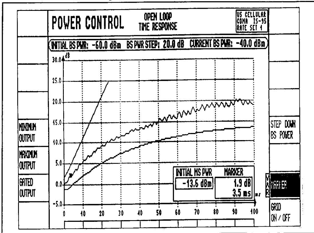
Figure 2.4.2.1 Test result for Test 1 (#1)
