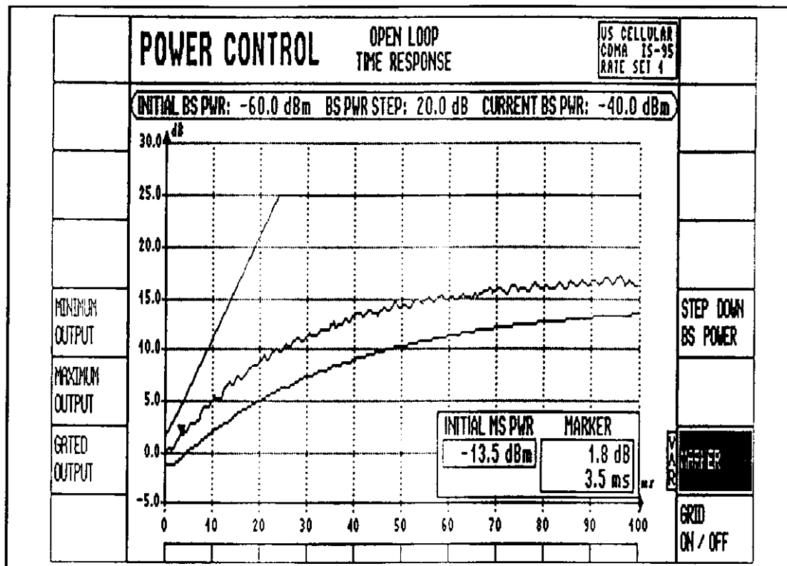
Figure 2.4.2.5 Test result for Test 1 (#2)
