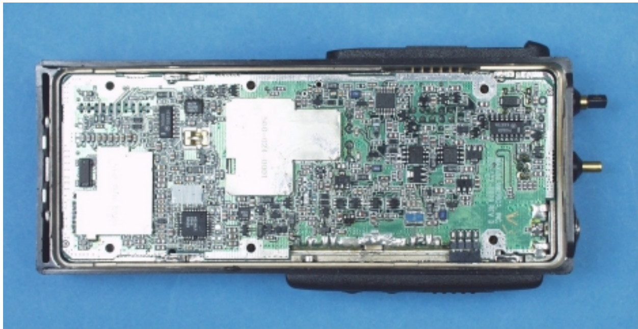
Circuit, Top
