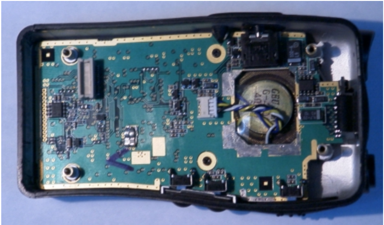
Digital Board – Back
