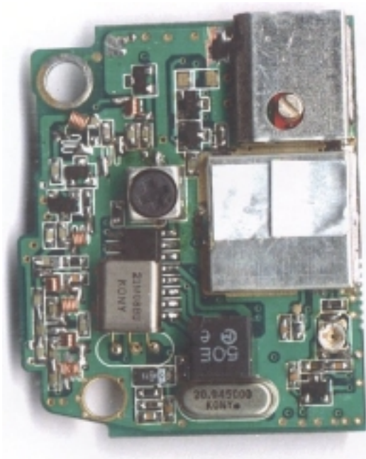
Sub PCB 2 With Shield
