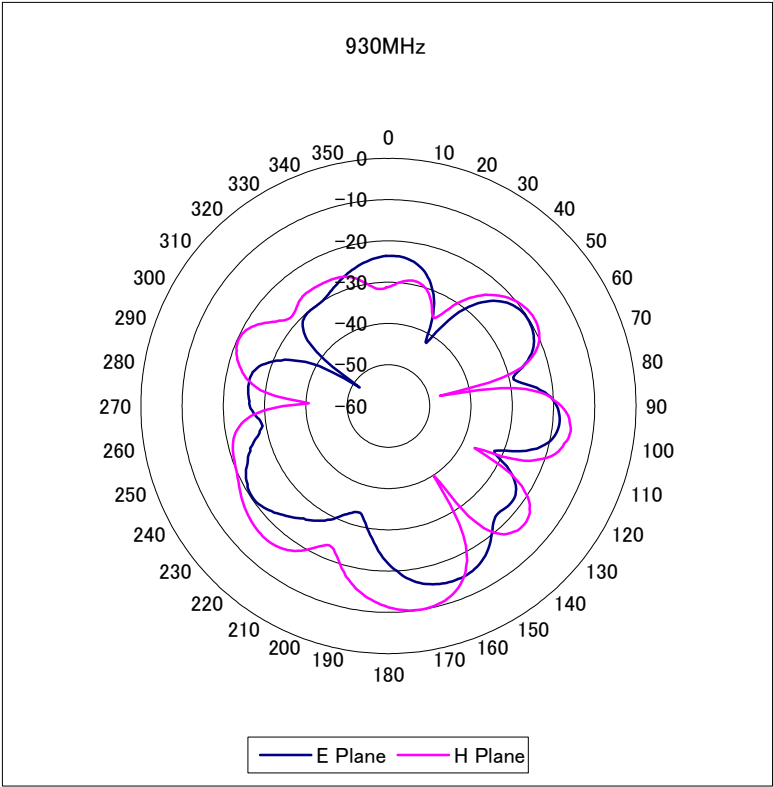
224E0500 2D Pattern[dBi] Y-Z
