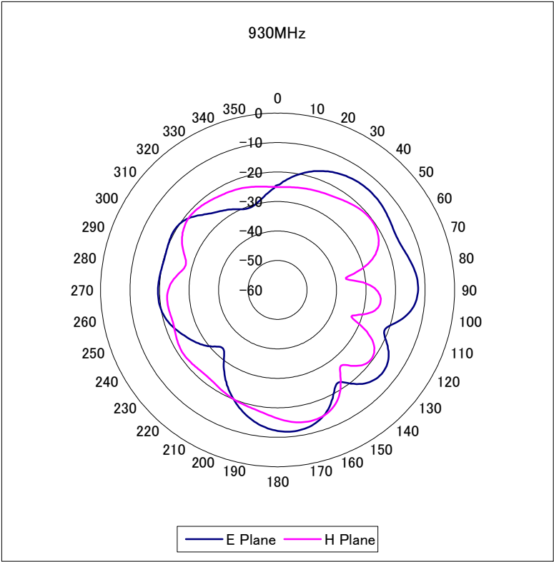
309E0901 2D Pattern [dBi] Y-Z
