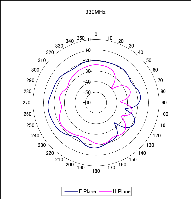
301E0901 2D Pattern [dBi] X-Y
