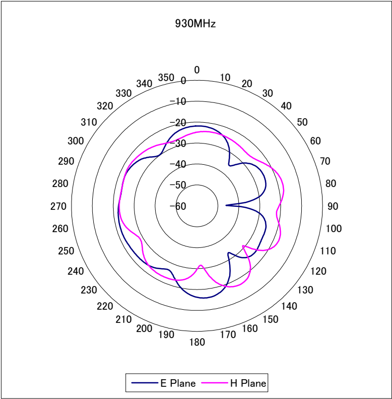
301E0901 2D Pattern [dBi] X-Z
