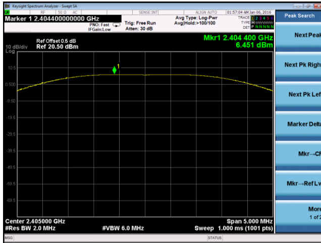
PWR-Zigbee 2405
