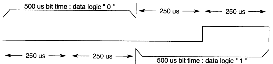
Figure 1 – Bit Timing
