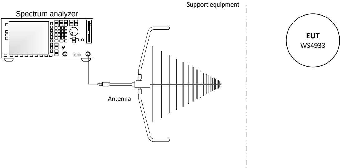
Figure 3.6-1: Setup diagram
