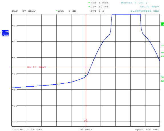
Figure 8.4-43: Radiated spurious emissions Lower band edge for 802.11n HT20, (TX 2417 MHz) – Average
