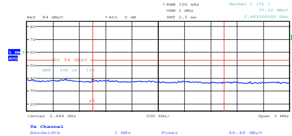
Figure 8.4-45: Radiated spurious emissions Upper band edge for 802.11b, (TX 2462 MHz) – Average
