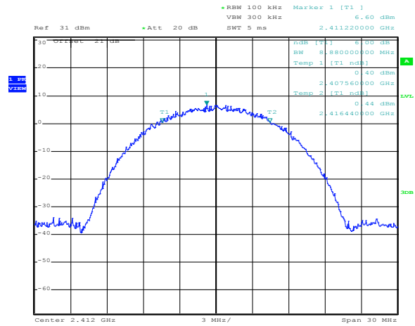
Figure 8.2-2: 6 dB bandwidth on 802.11b, sample plot – CCK: 11 Mbps
