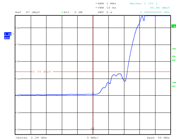
Figure 8.4-31: Radiated spurious emissions Lower band edge for 802.11b, (TX 2412 MHz) – Average
