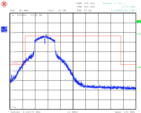
Figure 8.4-21: Conducted spurious emissions Lower band edge for 802.11n HT20, (TX 2417 MHz)
