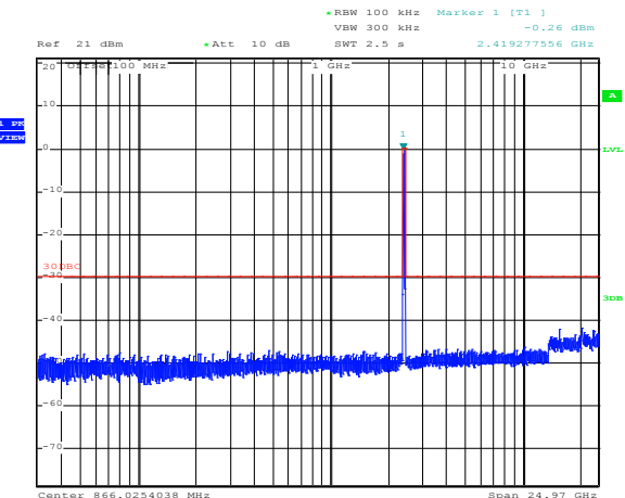
Figure 8.4-4: Conducted spurious emissions for 802.11n HT40 (TX 2422 MHz)
