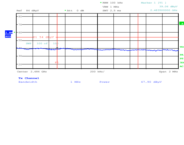
Figure 8.4-49: Radiated spurious emissions Upper band edge for 802.11n HT20, (TX 2462 MHz) – Average
