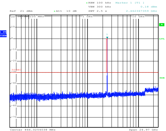
Figure 8.4-10: Conducted spurious emissions for 802.11g (TX 2462 MHz)
