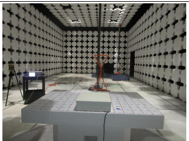
Spurious Emission Below 1GHz-Rear View
