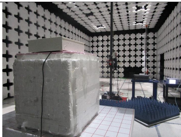
Spurious Emission Above 1GHz-Rear View
