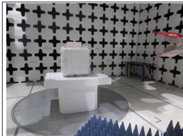
Spurious Emission Above 1GHz-Front View
