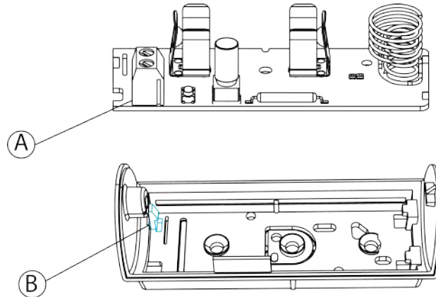
Figure 6: Removing the electronic board
