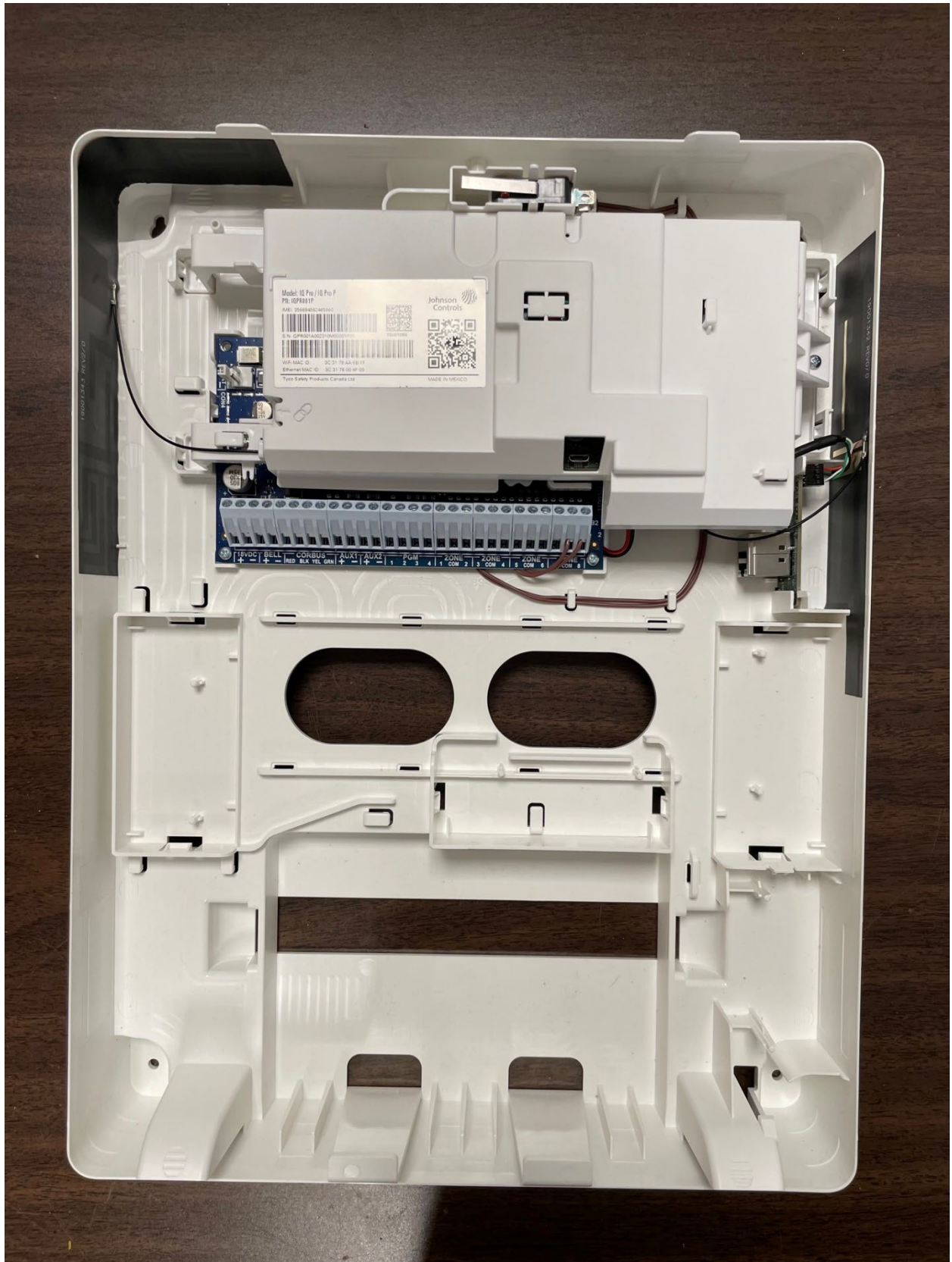
IQ Pro P Internal Photos
