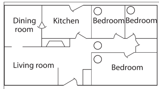
Figure 5 - Location of the detectors in units with only one bedroom area on one floor
