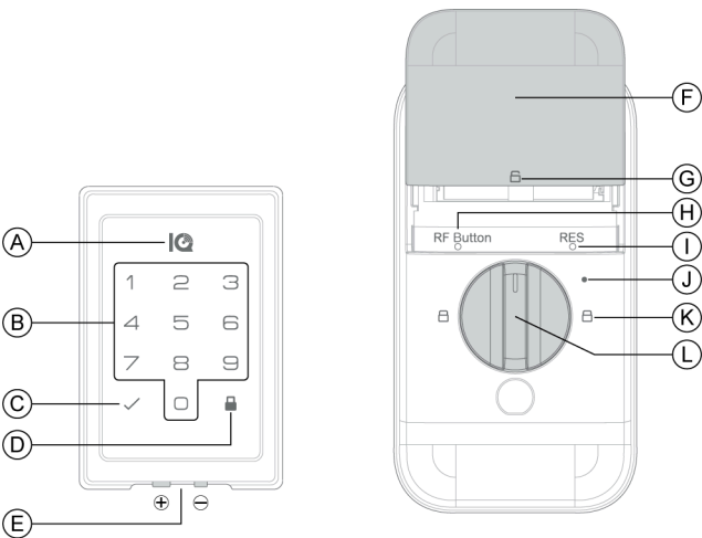
Figure 5: Smart lock overview
