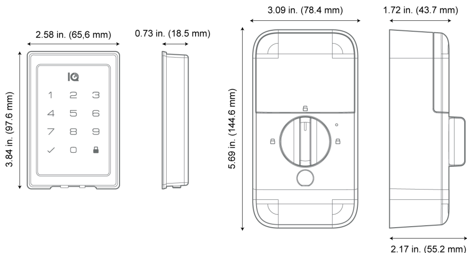
Figure 2: Smart lock dimensions
