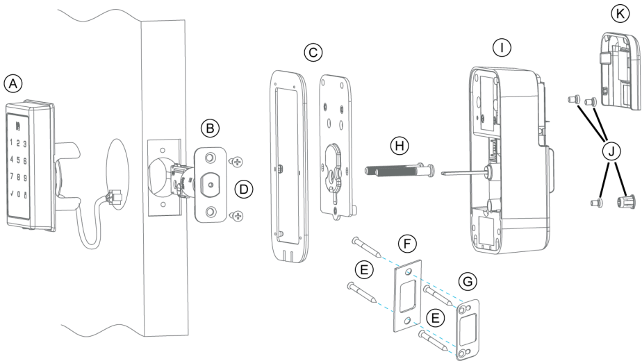
Figure 4: Smart lock installation overview
