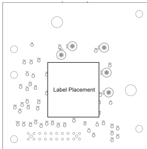
Label placement on back of PCB shown
