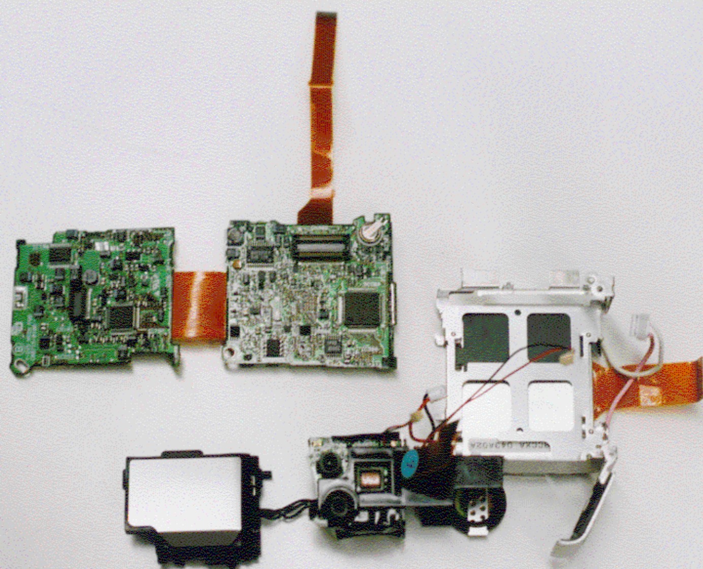
MAIN BOARD TAKEN OFF FinePix 6800Zoom FCC ID:F5GFP-6800 FUJI PHOTO FILM CO., LTD
