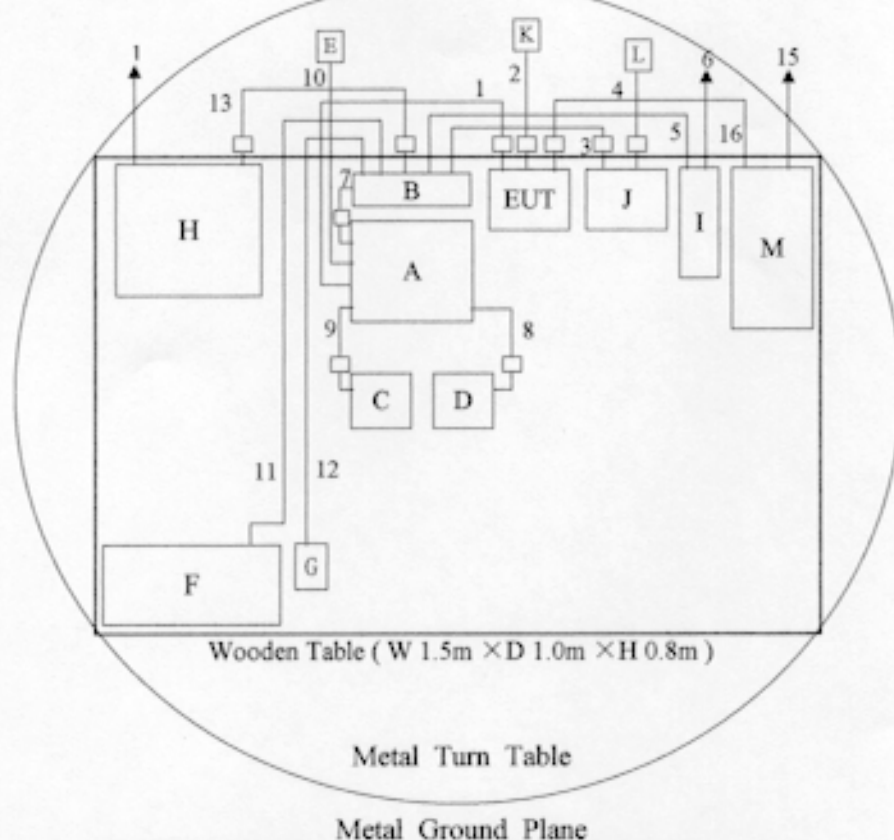
EUT's Test Arrangement of Radiation Non Metallic (F. R. P.) Dome ( W 8.0m × D 6.3m × H 5.5m )
