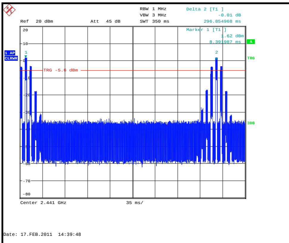
Channel repetition time – 2Mbps
