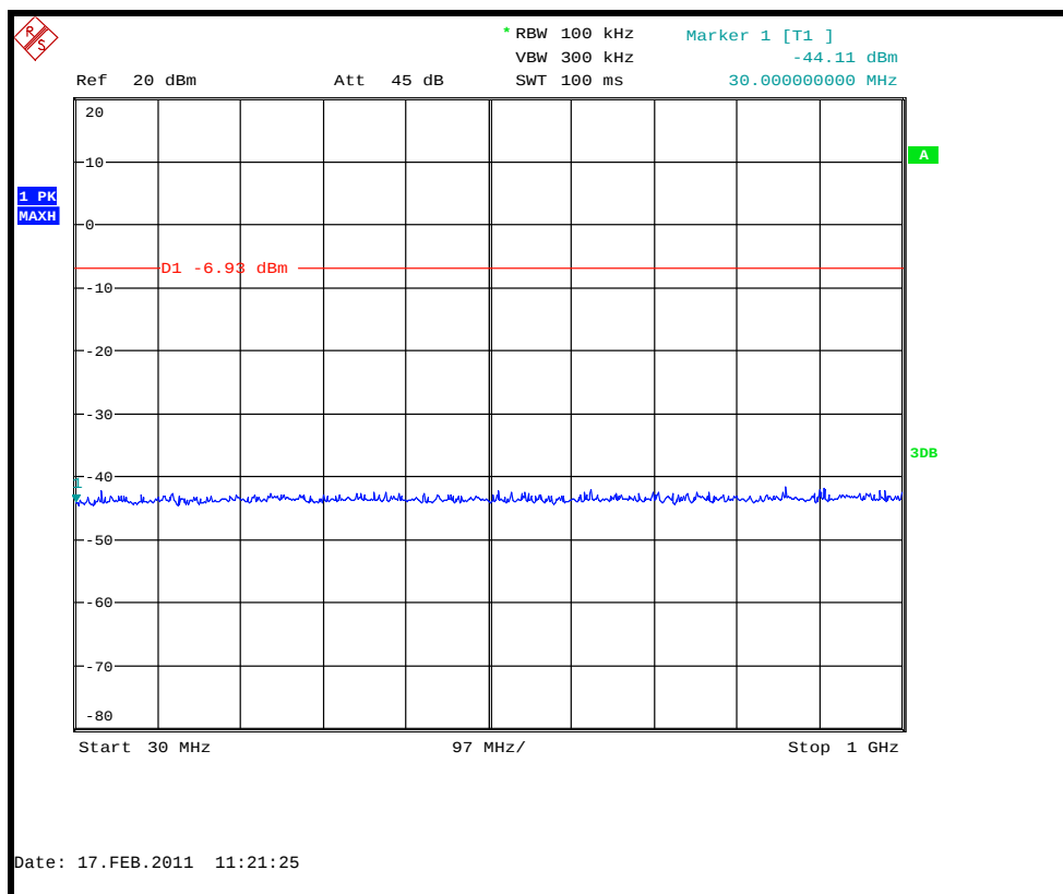
Conducted Spurious emissions 30 MHz to 1 GHz – 2480.0MHz – 1Mbps
