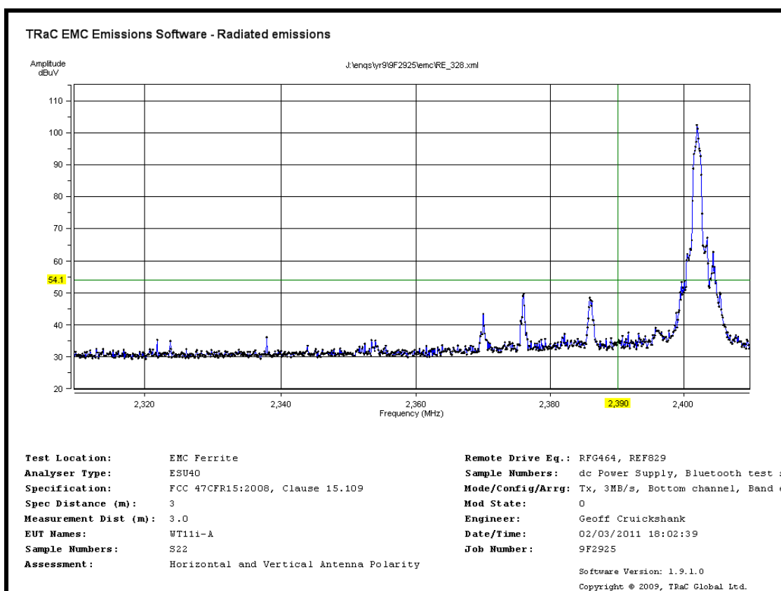
Lower Bandedge
