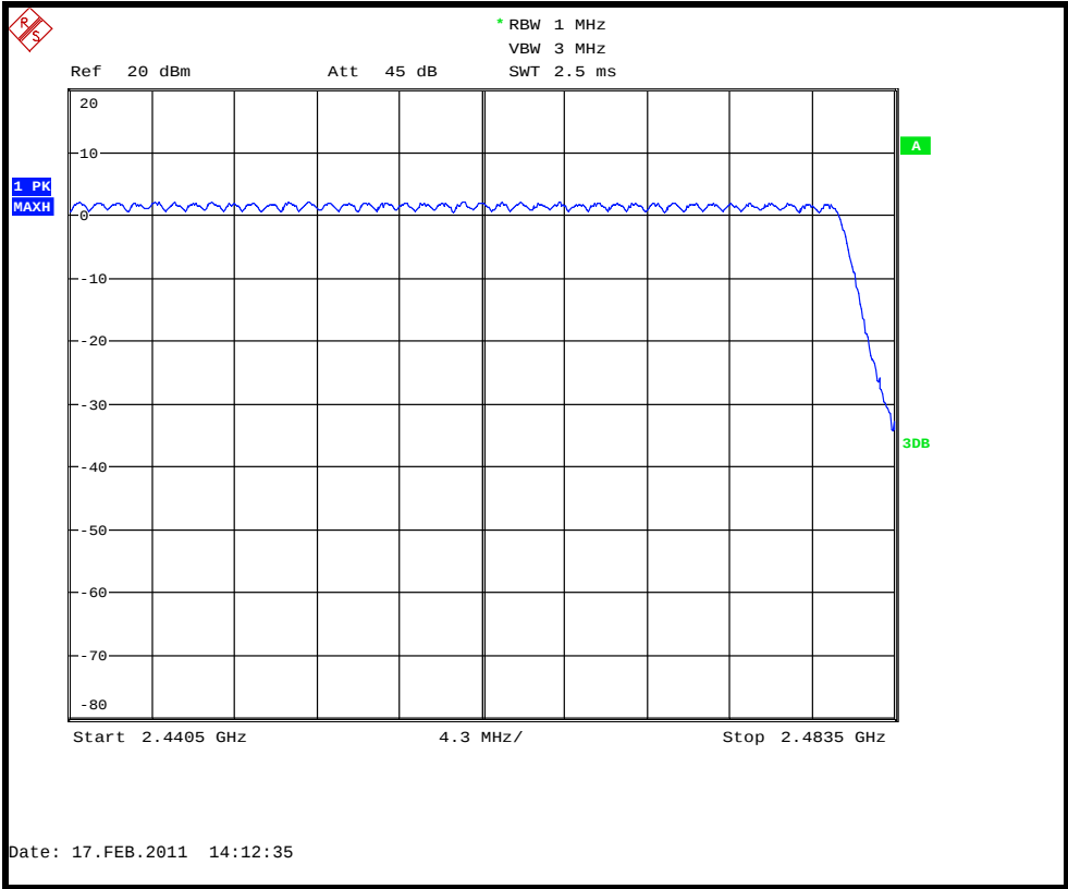
Number of Hopping Channels – 2Mbps
