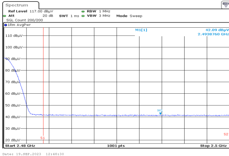
2480.0 F3 RestrictedBand Horizontal AVG
