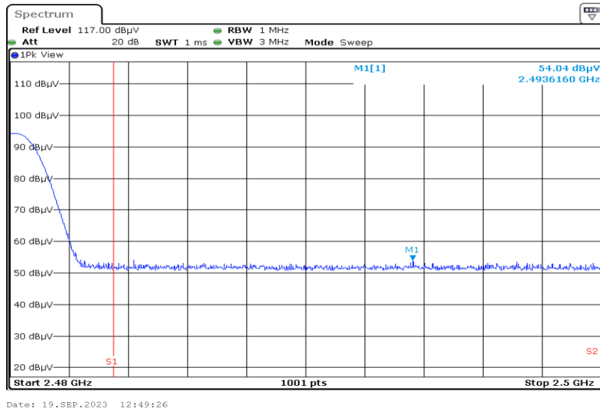
2480.0 F3 RestrictedBand Horizontal PEAK
