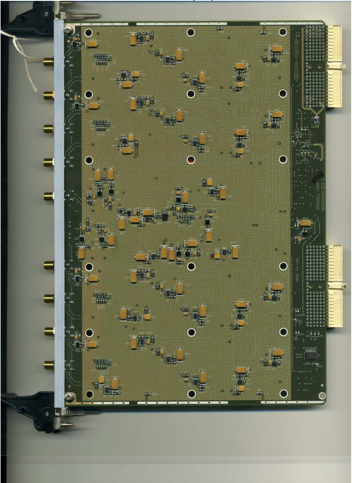
Hub Down Converter (HDC) Back
