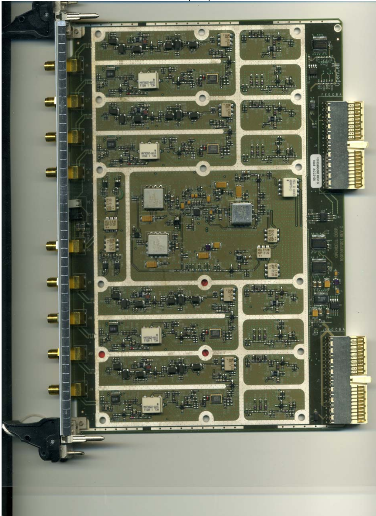
Hub Down Converter (HDC) Front – View 2
