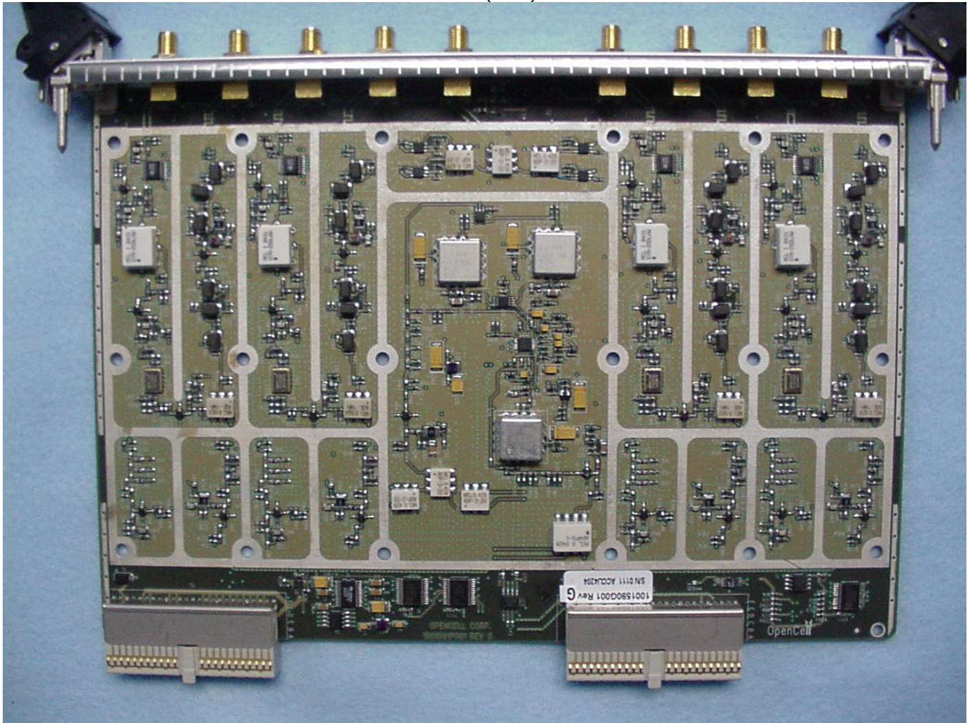
Hub Down Converter (HDC) Front – View 1
