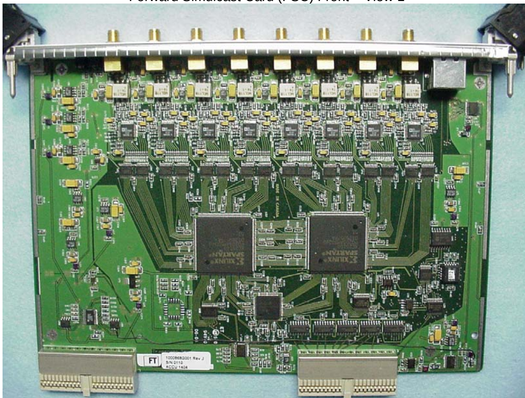
Forward Simulcast Card (FSC) Front – View 2
