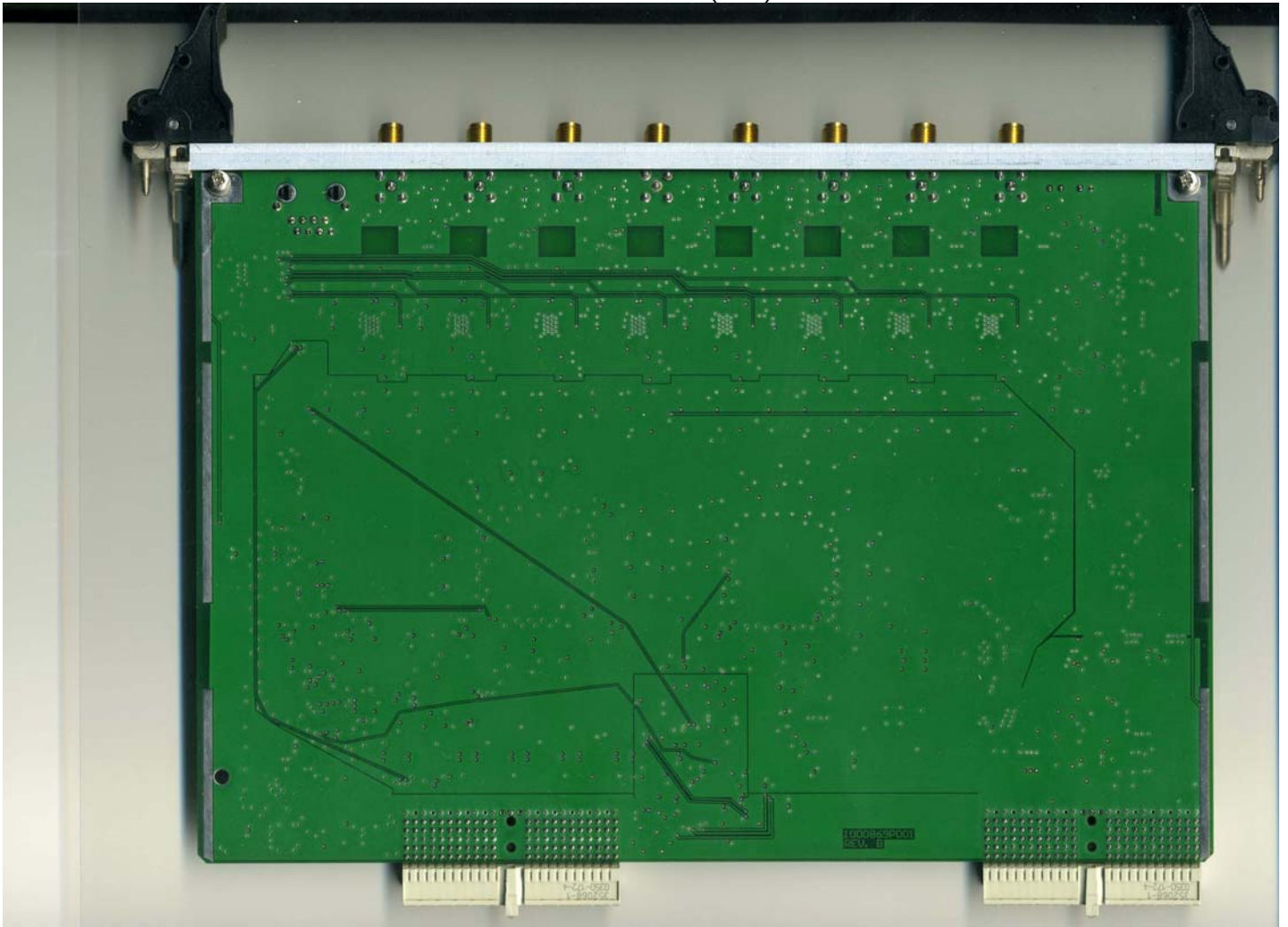
Forward Simulcast Card (FSC) Back
