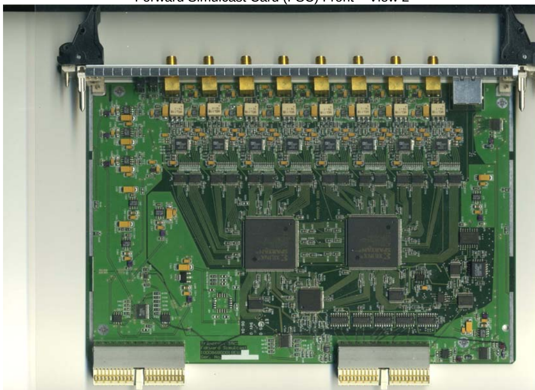
Forward Simulcast Card (FSC) Front – View 2
