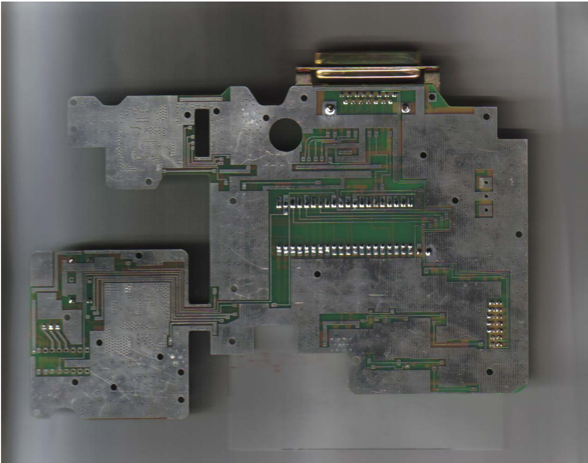
Broadband 10W LPA 0071-2300 Bottom
