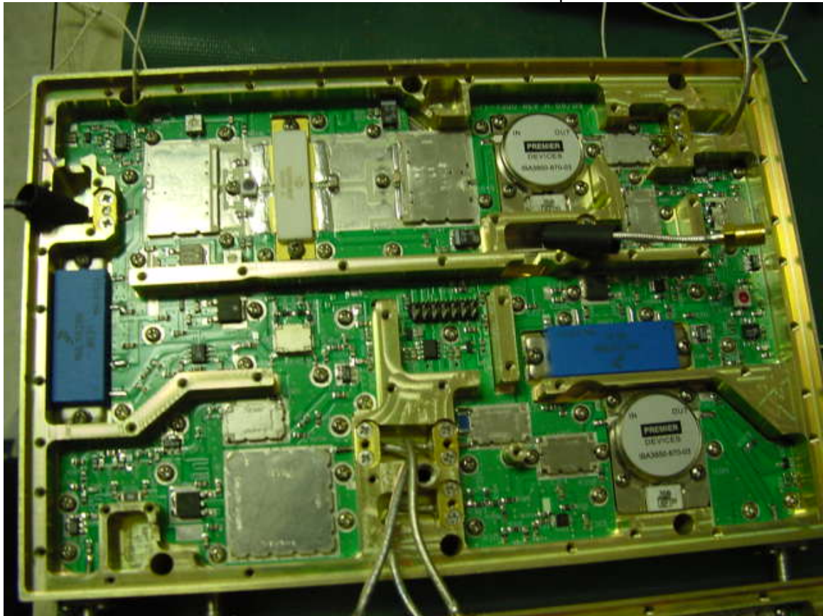
Broadband 10W LPA 0071-1300 Top
