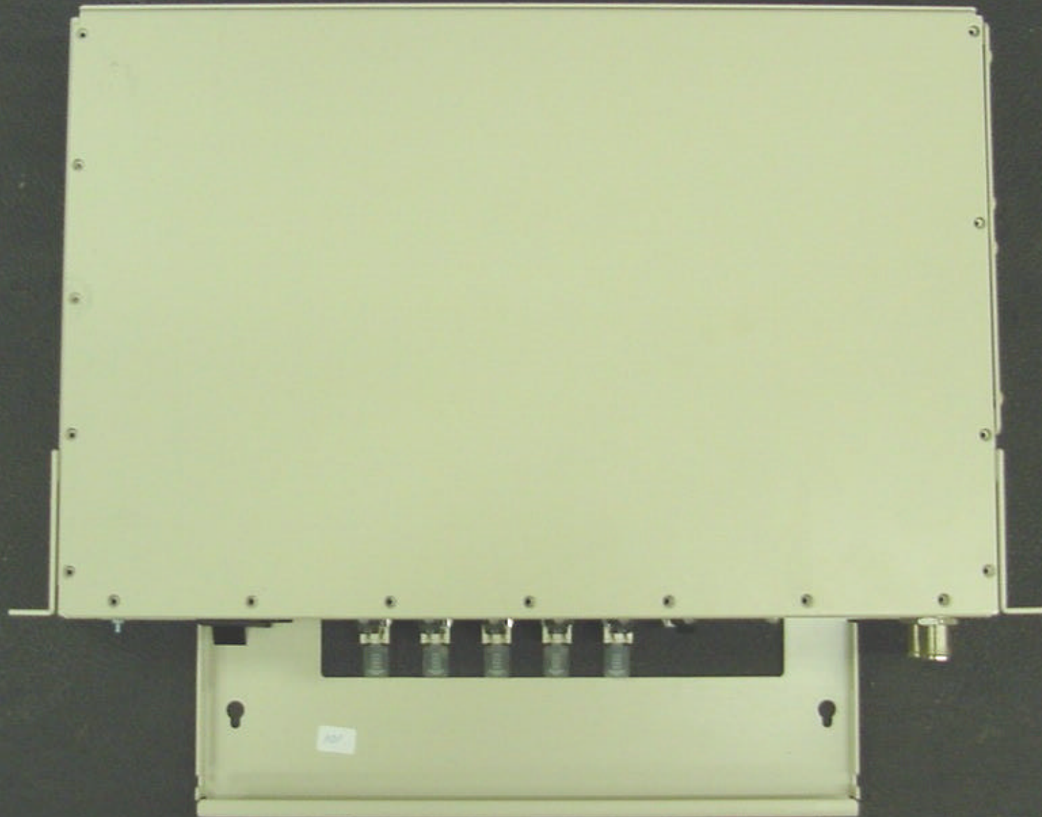
Digivance ICS SMR DHU Top View
