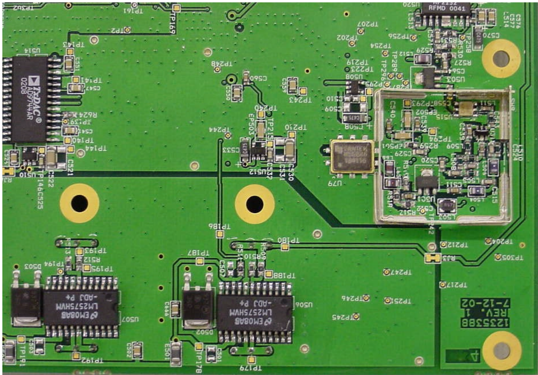
Digivance ICS SMR DRU Control Board - B2
