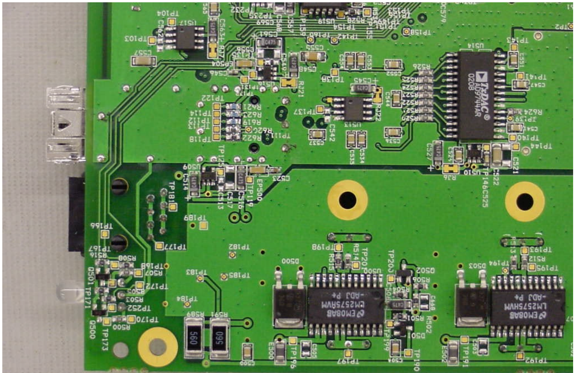
Digivance ICS SMR DRU Control Board - B1
