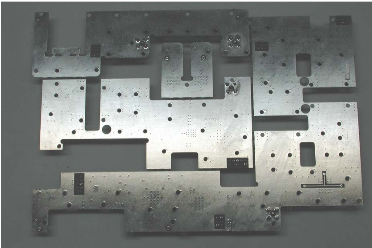
Digivance 800 MHz 20 Watt LPA RF Board Bottom View
