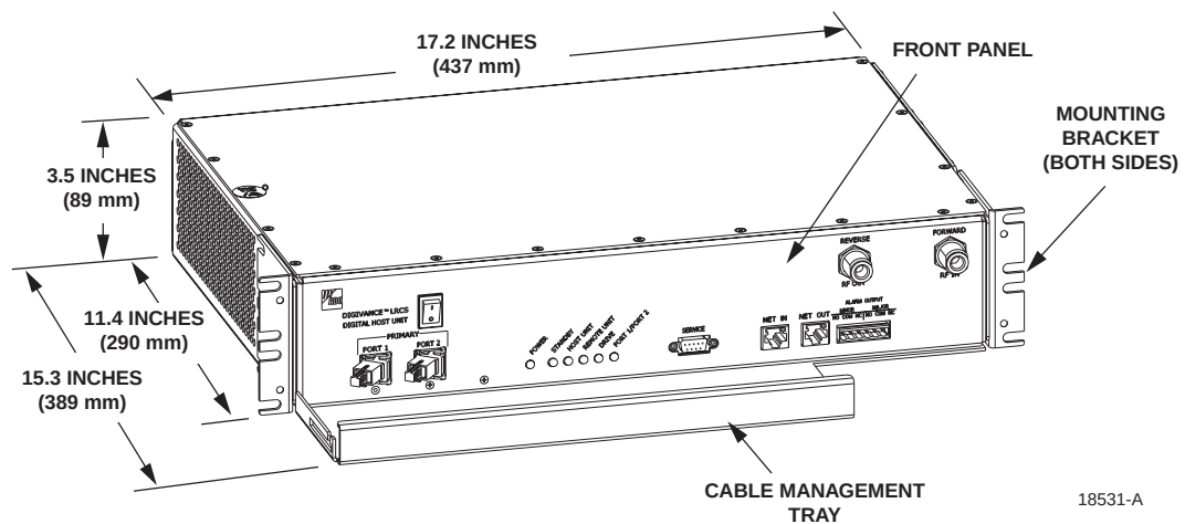
Figure 2-1. Host Unit
