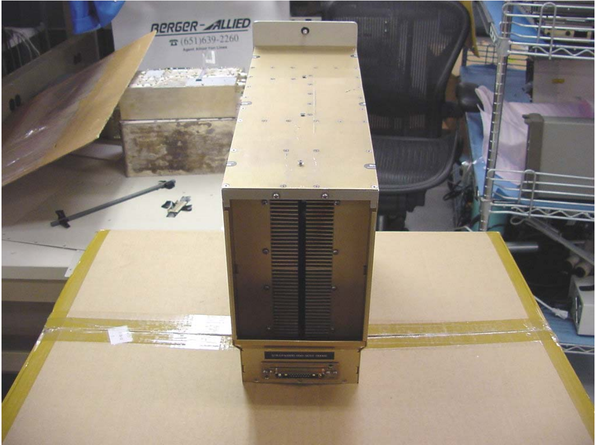
800 MHz Linear Power Amplifier Rear View
