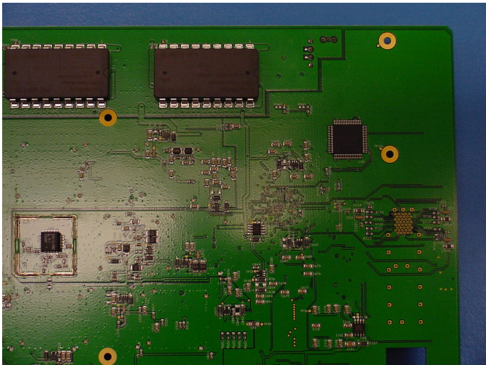
Digivance LRCS 800 MHz Host Board Bottom View 3
