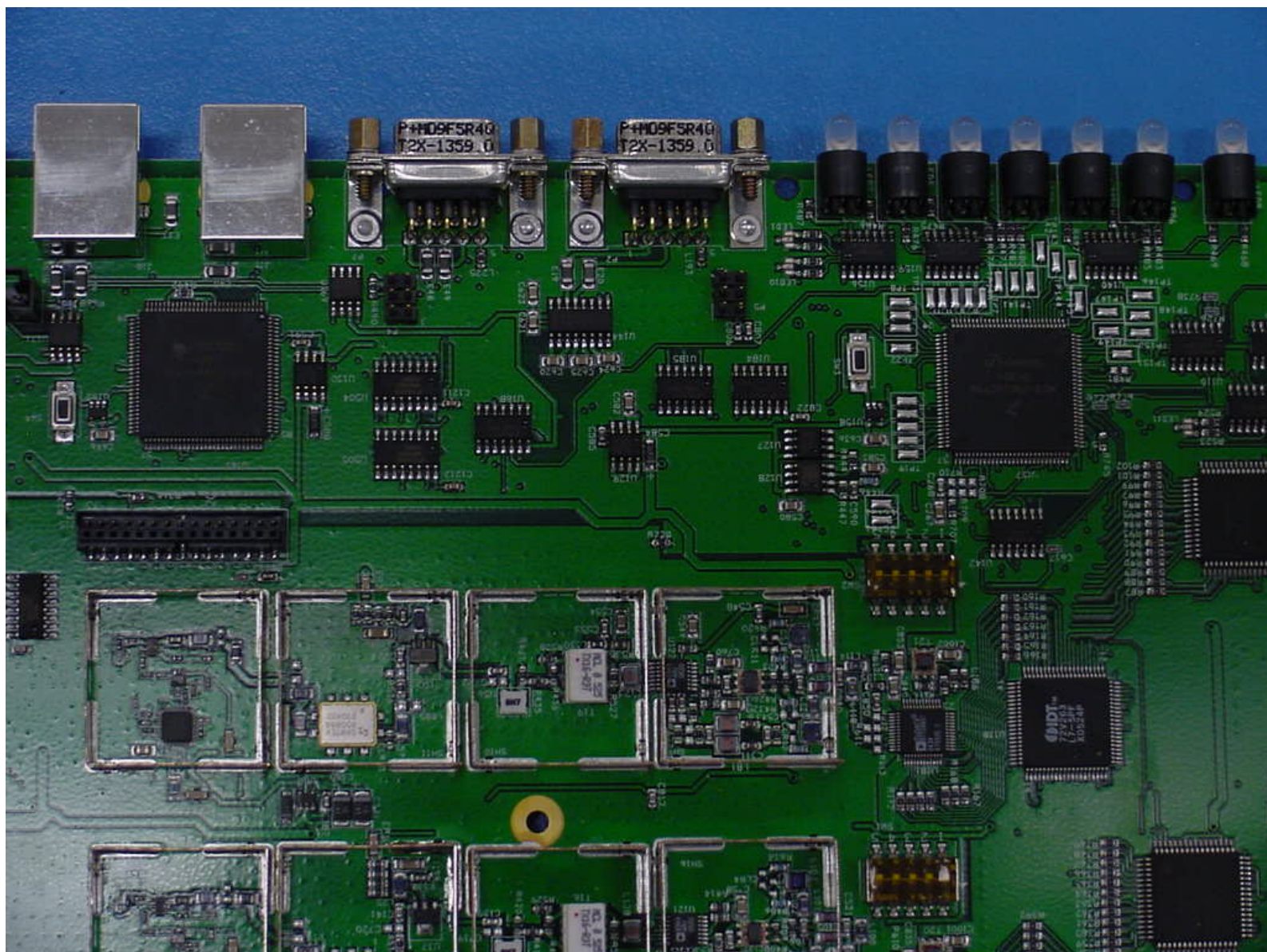
Digivance LRCS 800 MHz Host Board Top View 7
