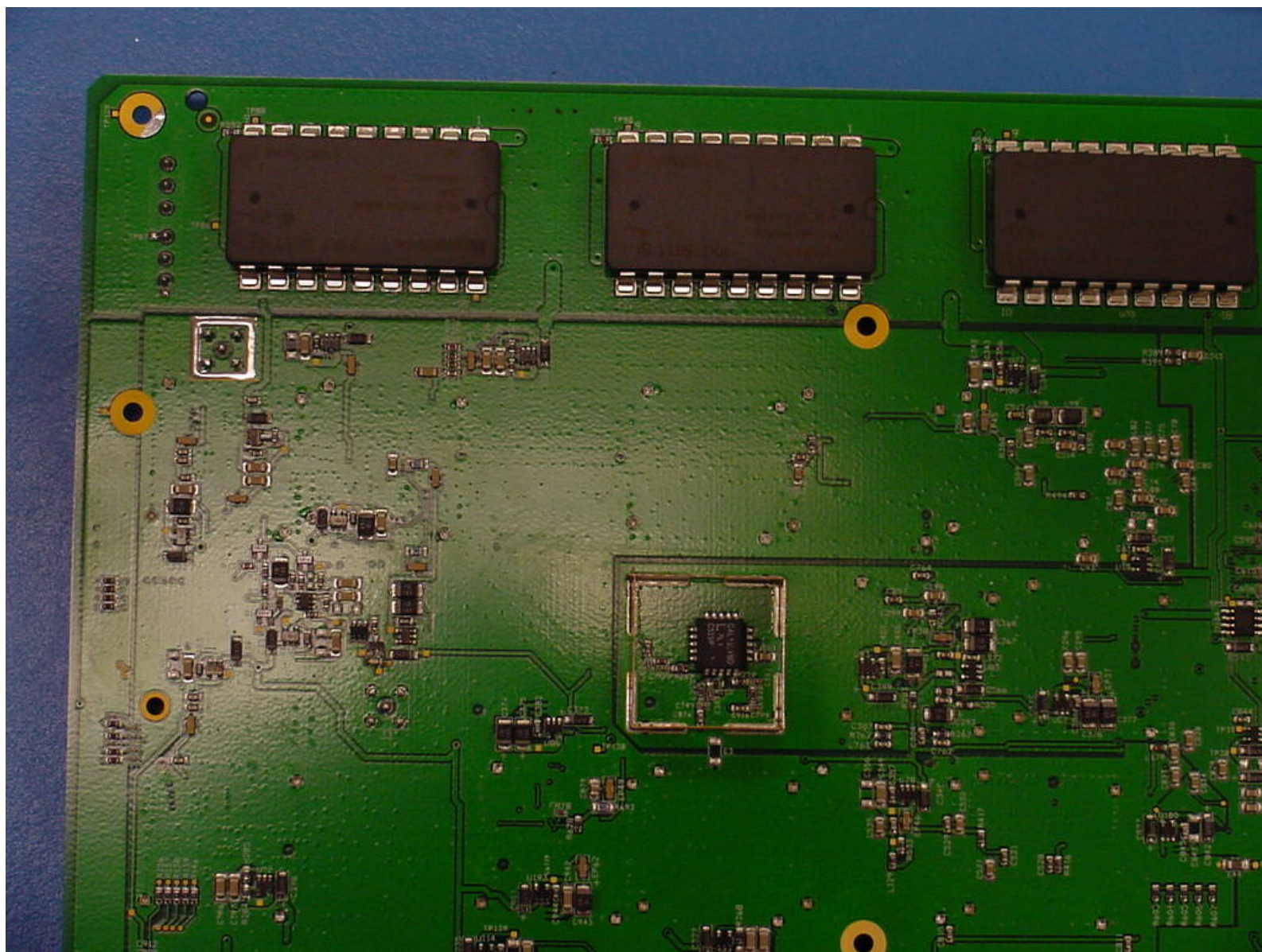
Digivance LRCS 800 MHz Host Board Bottom View 4
