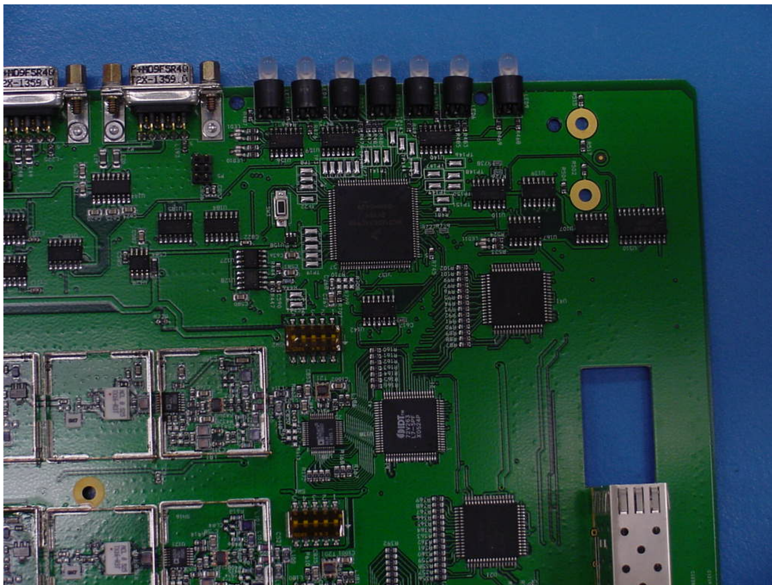
Digivance LRCS 800 MHz Host Board Top View 8
