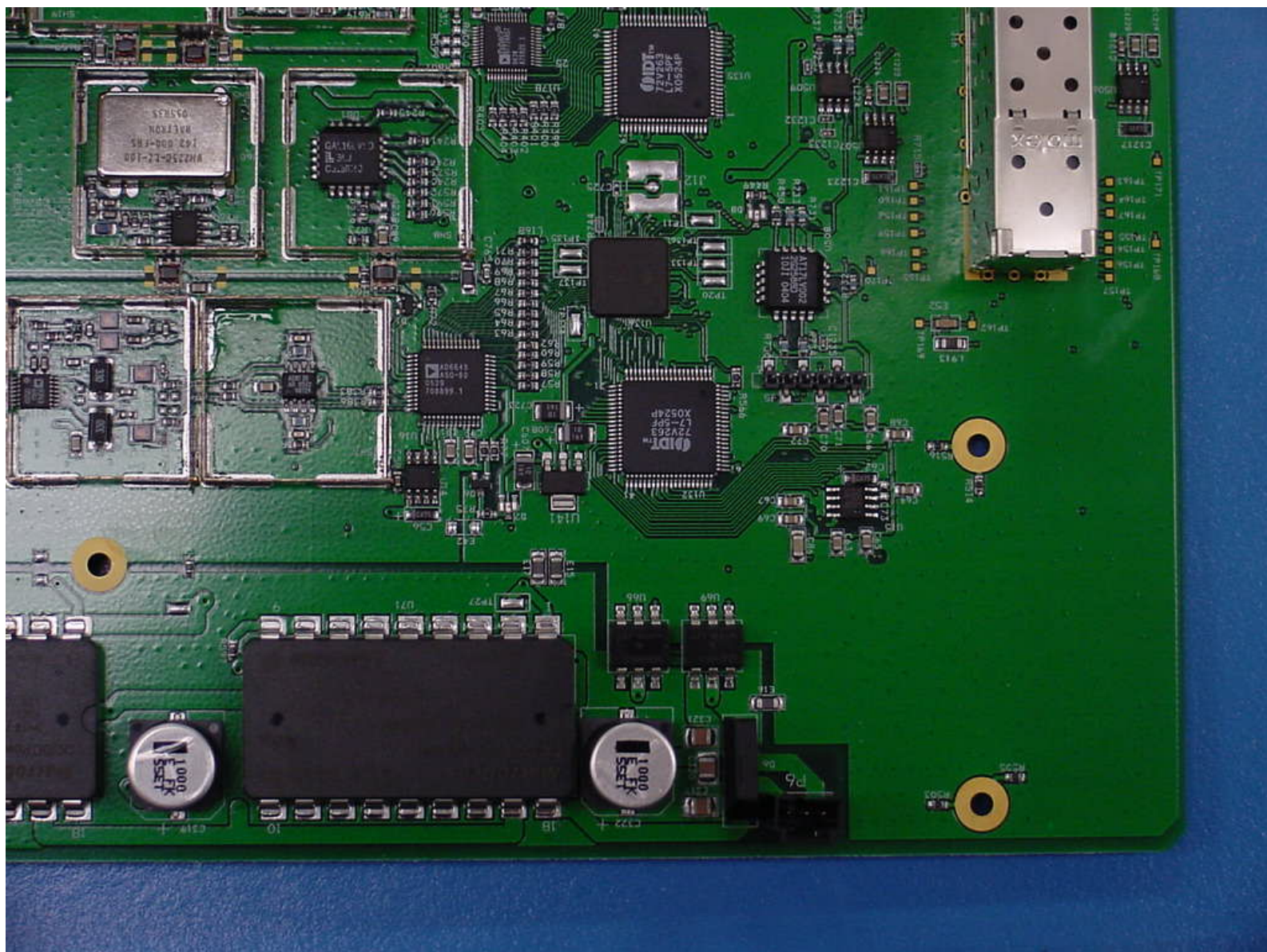
Digivance LRCS 800 MHz Host Board Top View 2
