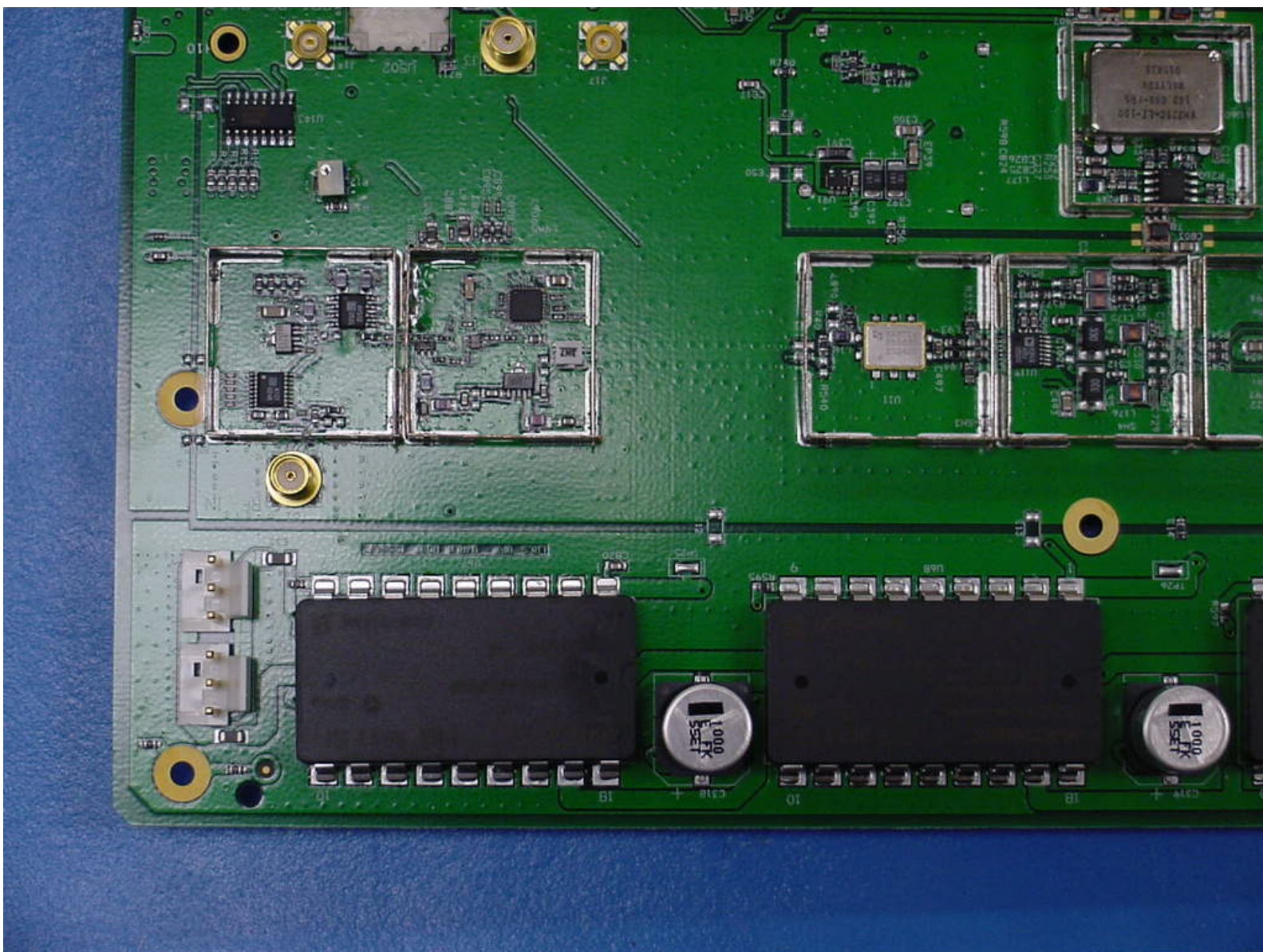
Digivance LRCS 800 MHz Host Board Top View 1
