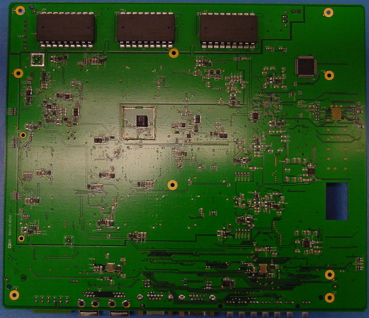
Digivance LRCS 800 MHz Host Board Bottom View
