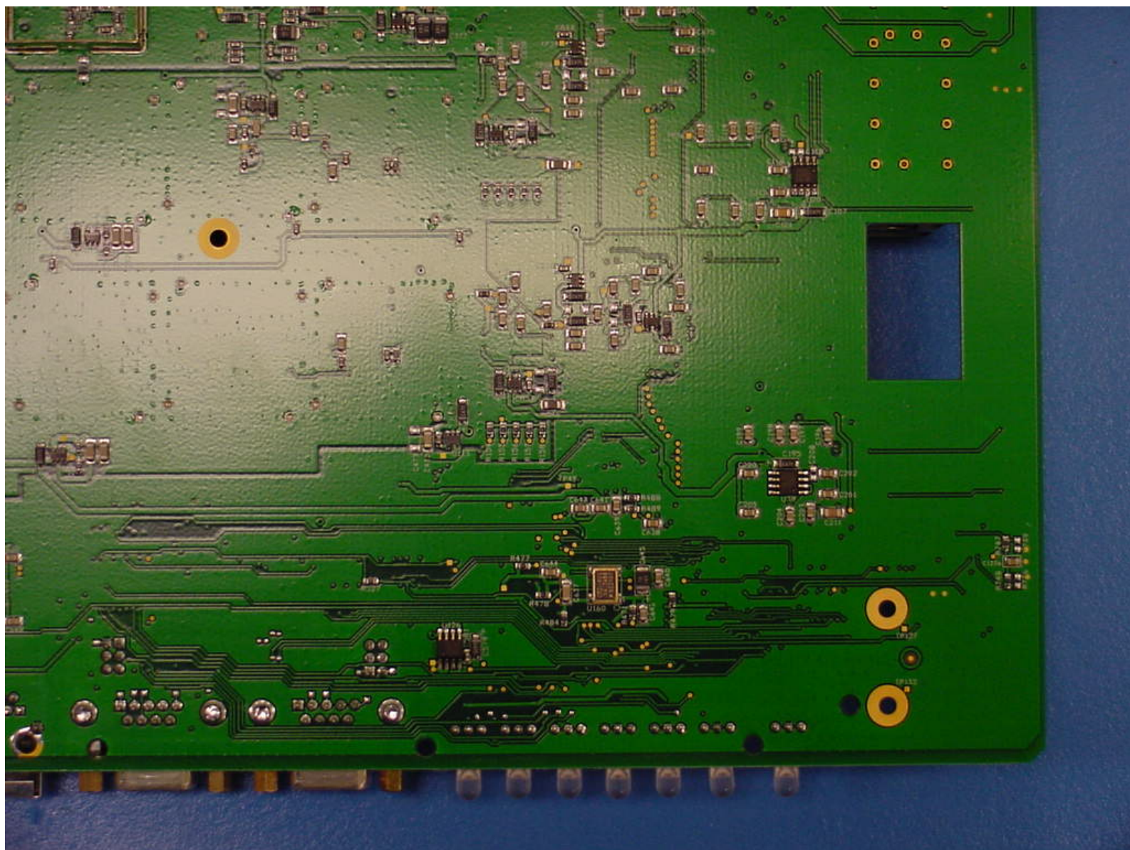
Digivance LRCS 800 MHz Host Board Bottom View 2
