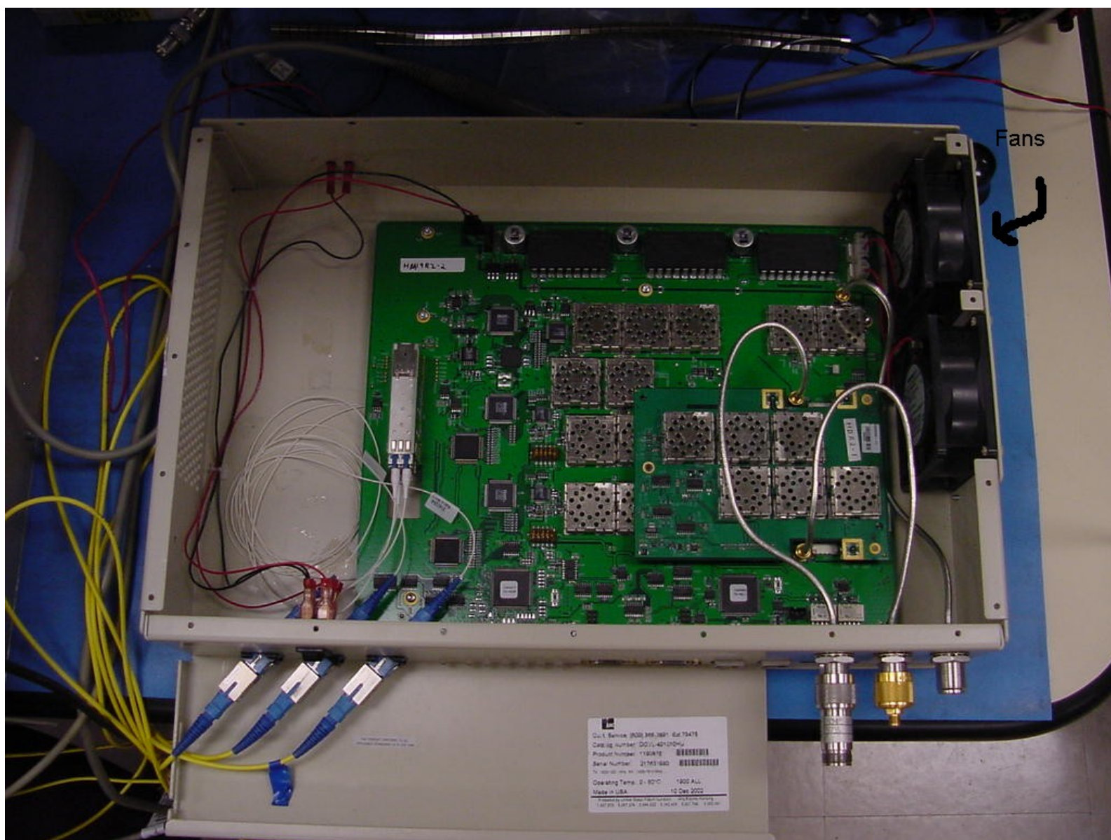
Digivance LRCS 800 MHz Host Unit Open Top View
