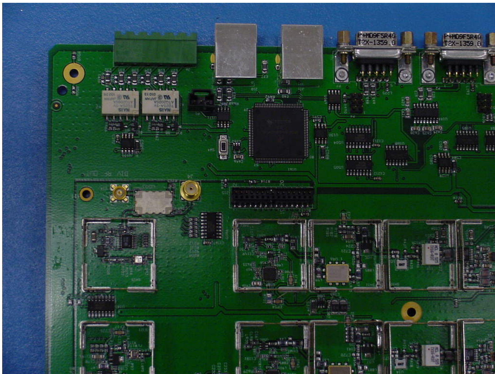
Digivance LRCS 800 MHz Host Board Top View 6
