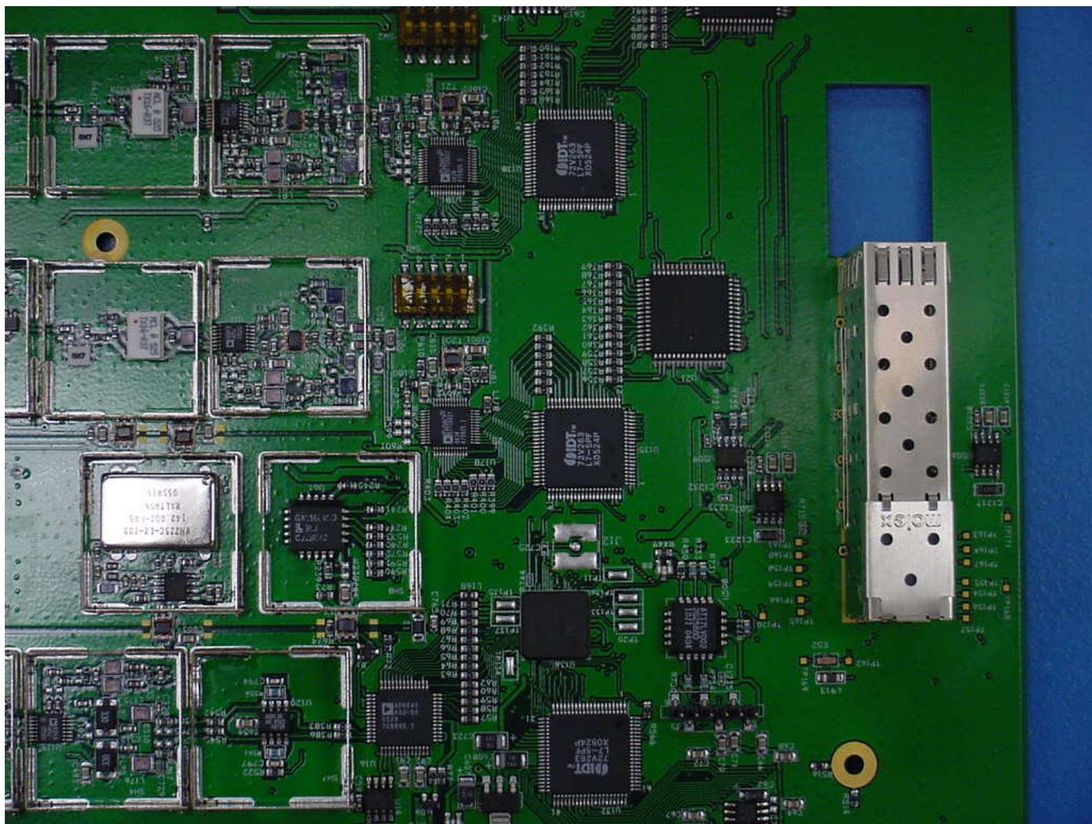
Digivance LRCS 800 MHz Host Board Top View 3
