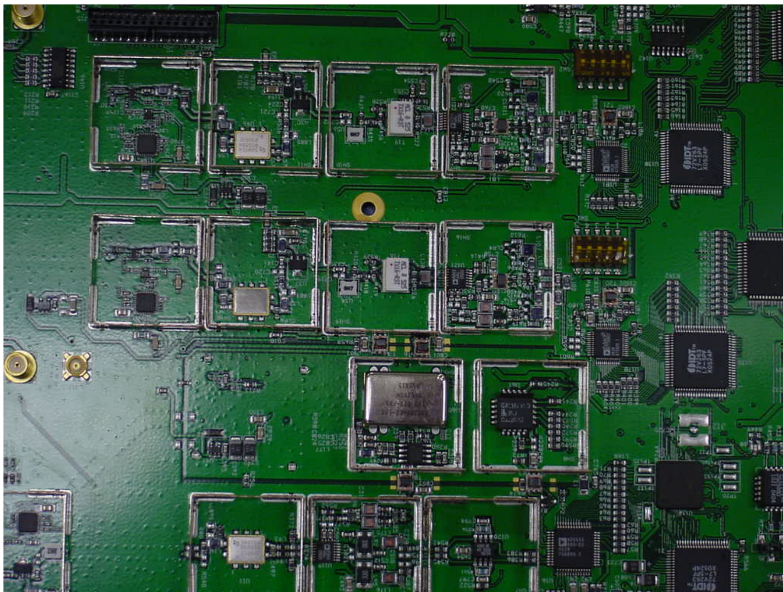
Digivance LRCS 800 MHz Host Board Top View 4
