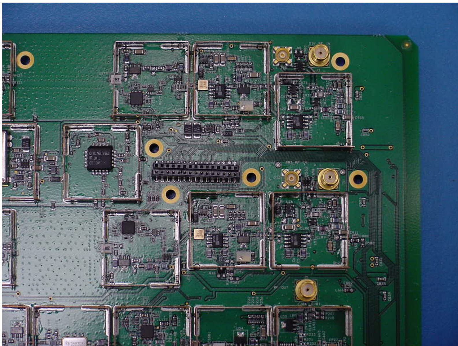
Digivance LRCS 800 MHz STM Board Top View 4
