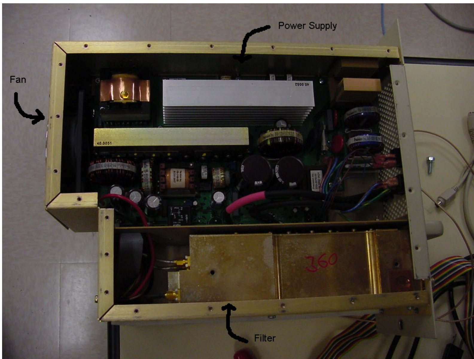
Digivance LRCS 800 MHz Signal Transport Module – STM Open Left View
