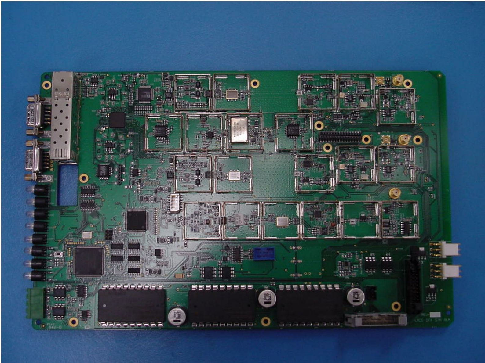
Digivance LRCS 800 MHz STM Board Top View
