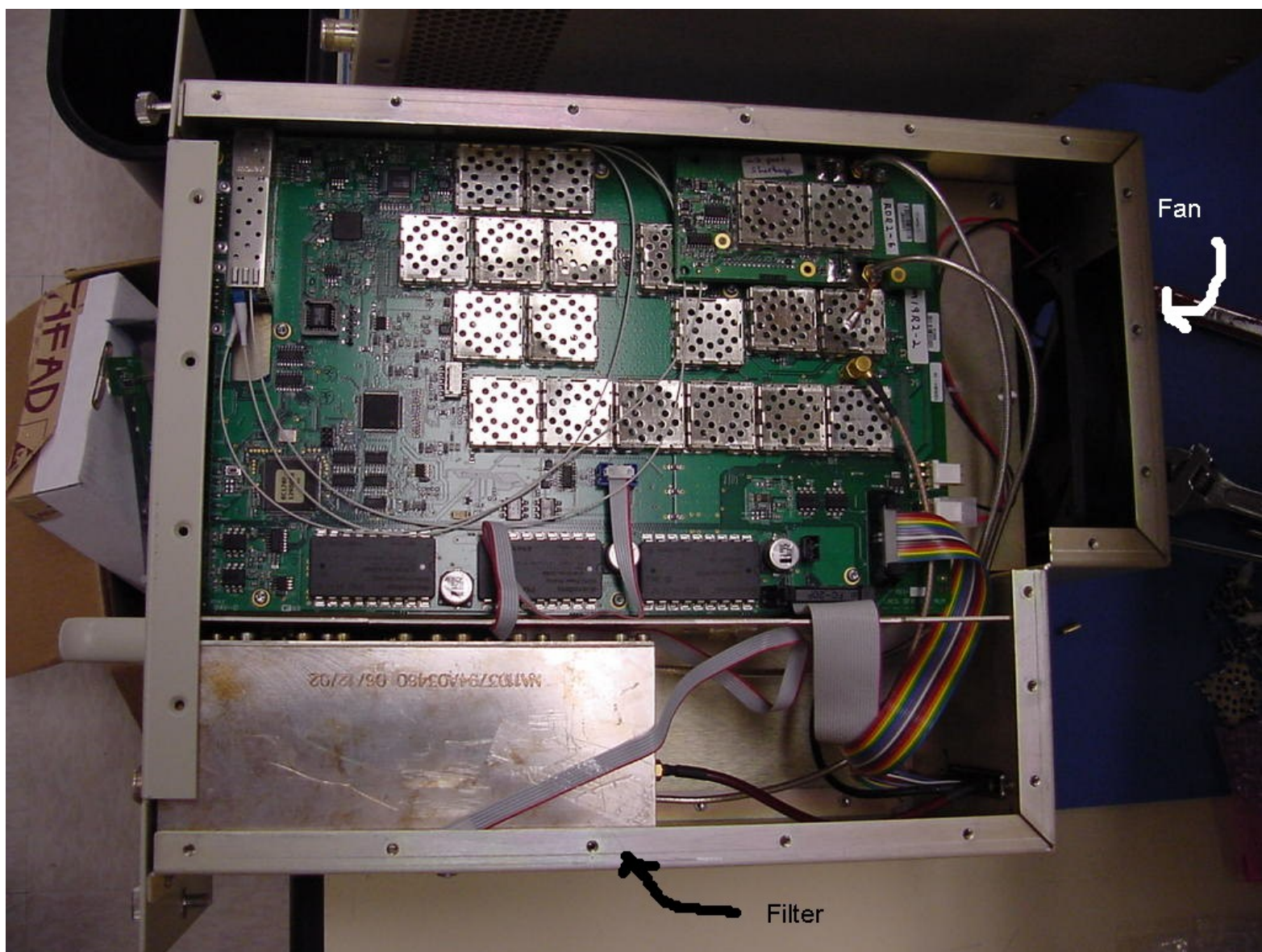
Digivance LRCS 800 MHz Signal Transport Module – STM Open Right View
