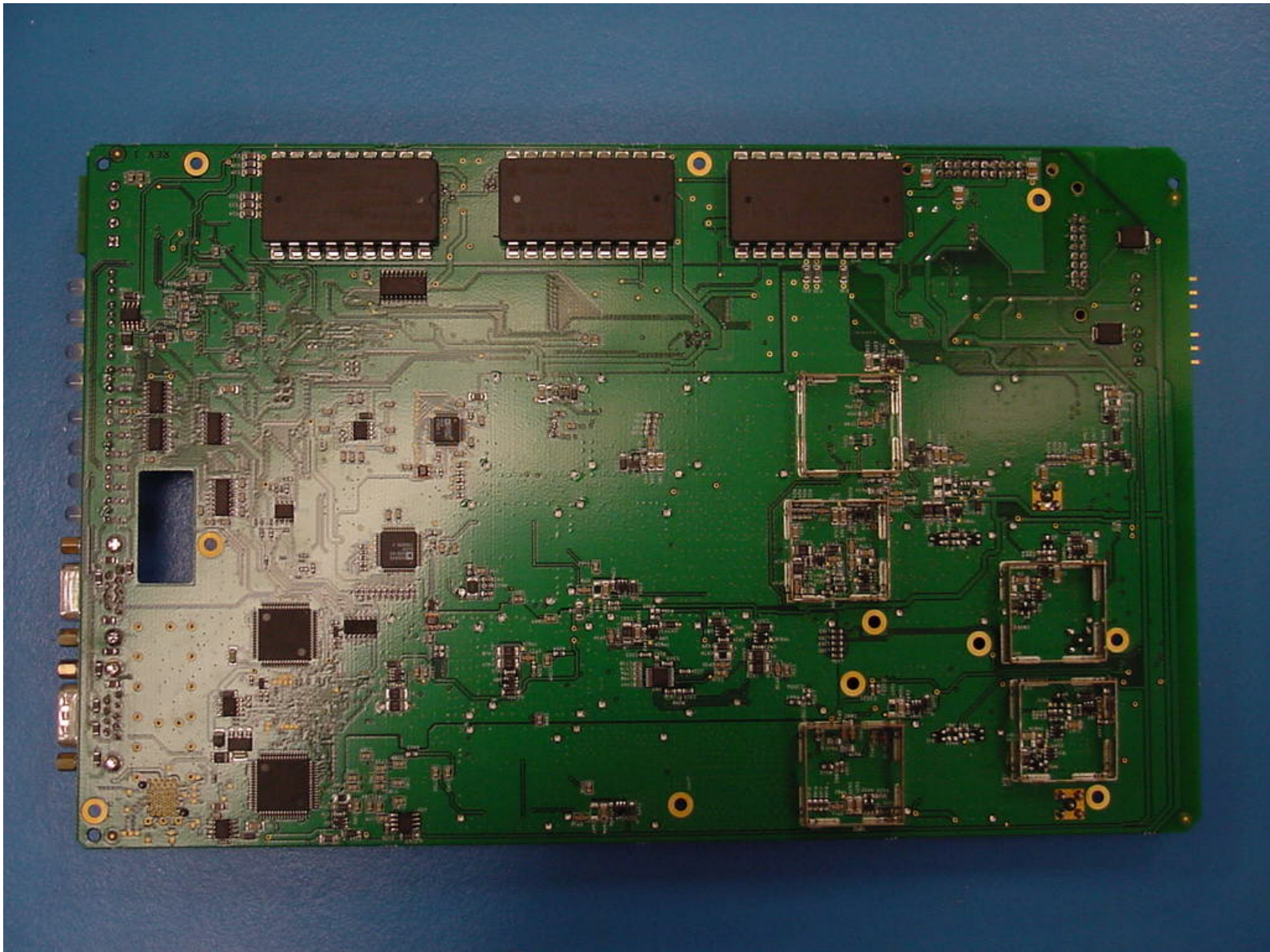
Digivance LRCS 800 MHz STM Board Bottom View
