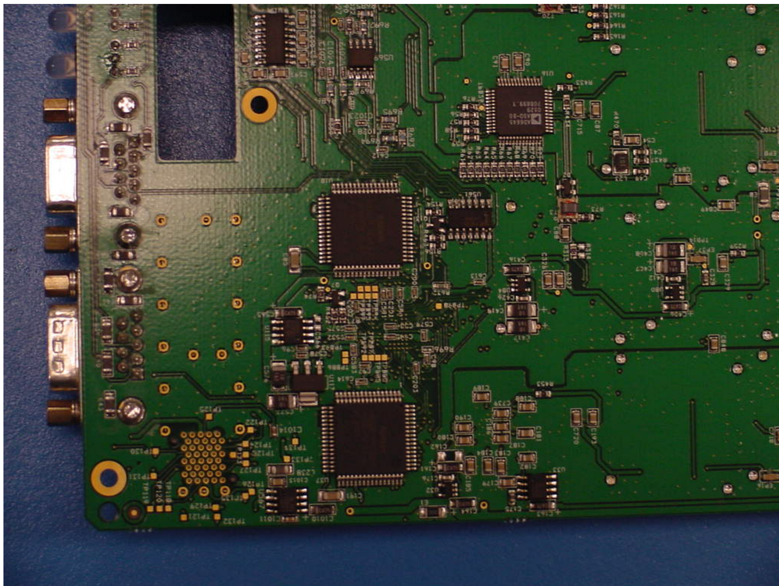
Digivance LRCS 800 MHz STM Board Bottom View 1
