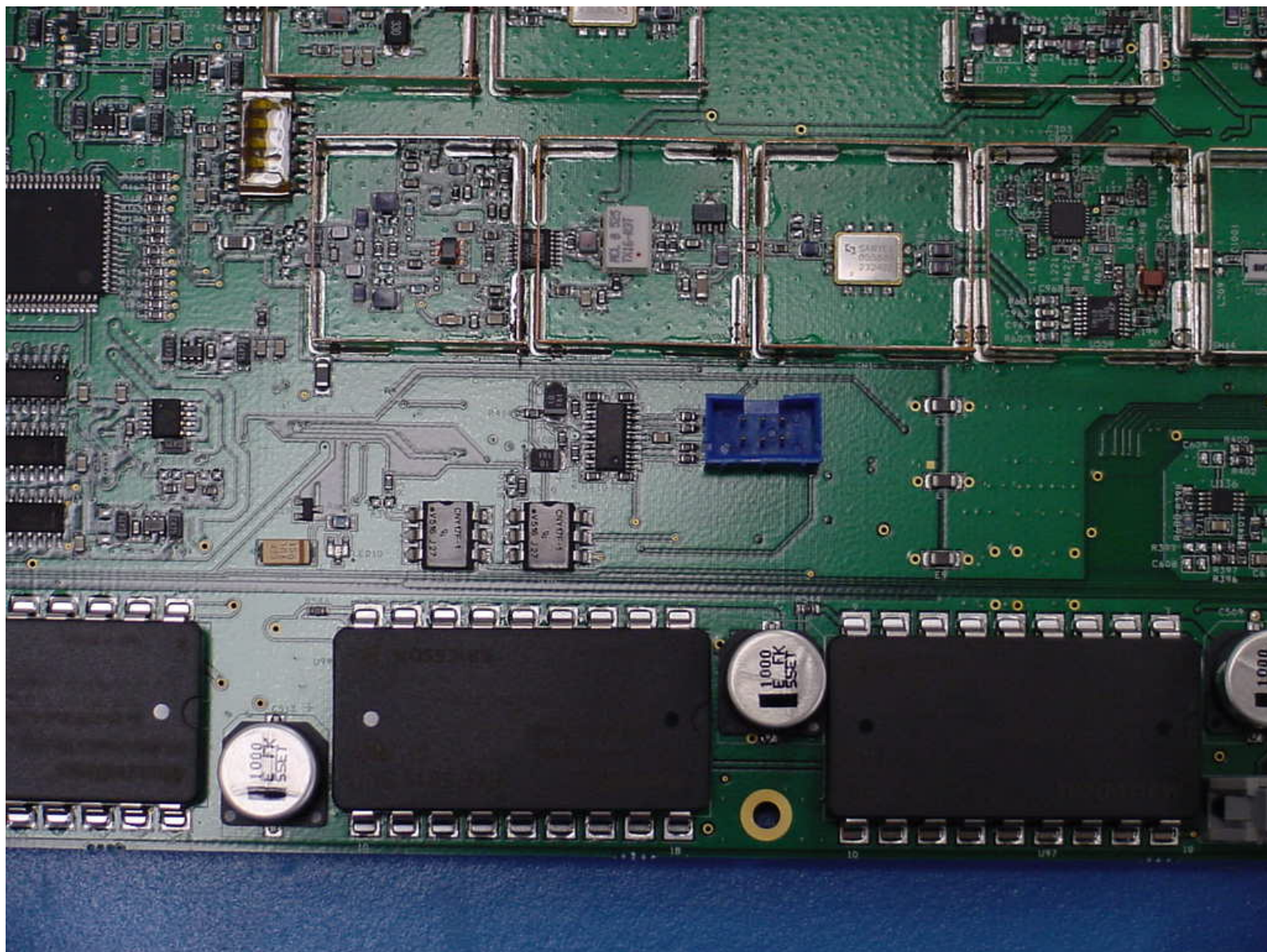
Digivance LRCS 800 MHz STM Board Top View 2
