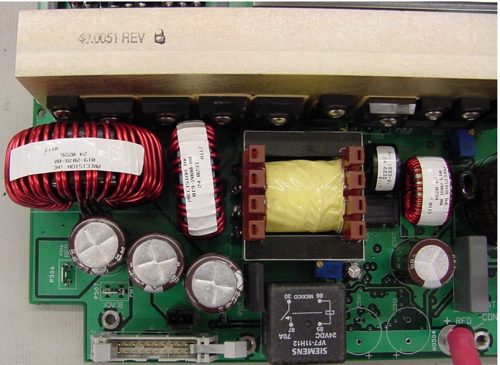
Digivance LRCS Power Supply Board Top View - Lower Left
