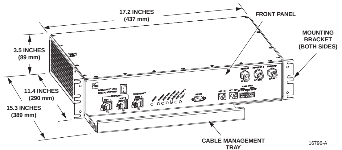
Figure 2-1. Host Unit
