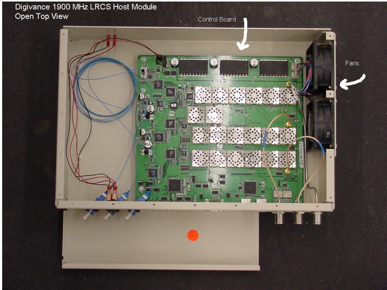
Digivance LRCS 1900 MHz Host Control Board Top View
