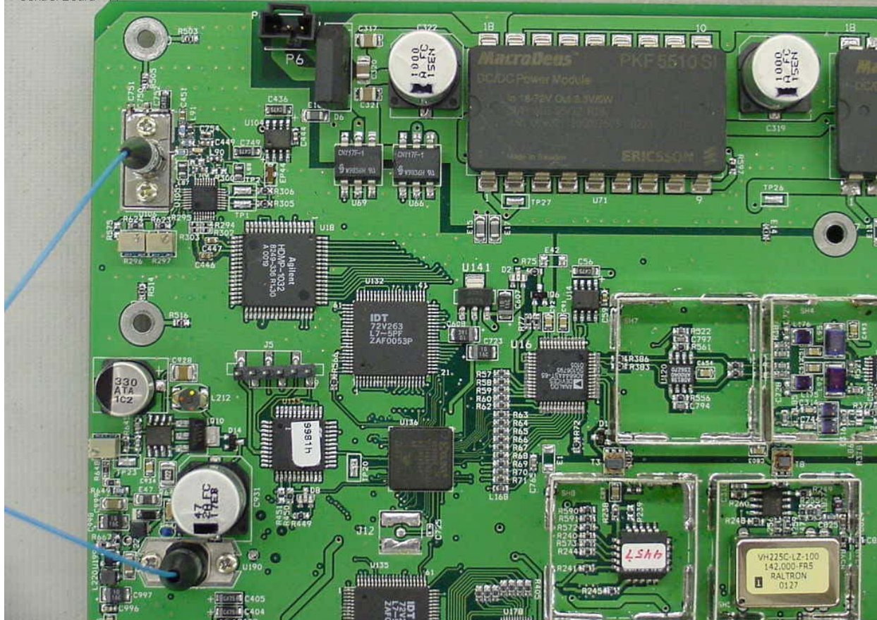
Digivance LRCS 1900 MHz Host Control Board - T7
