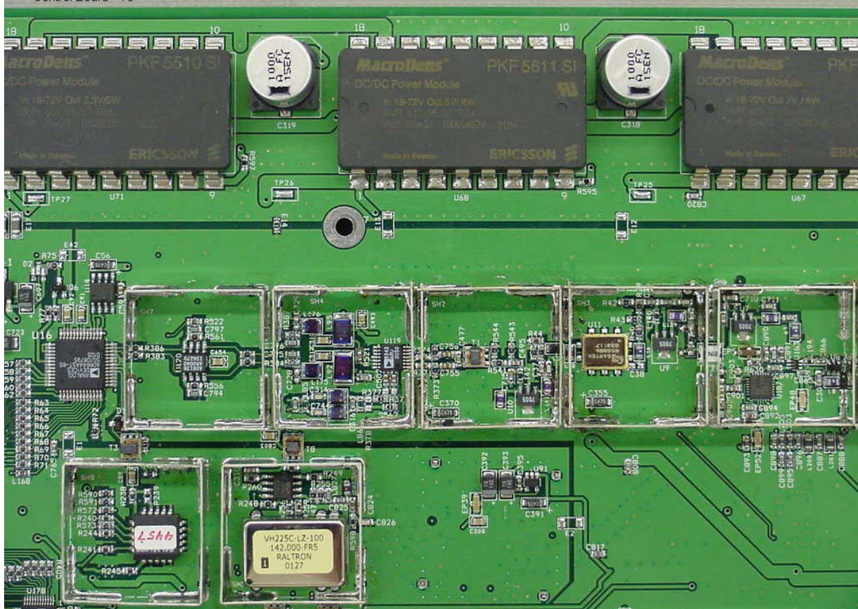
Digivance LRCS 1900 MHz Host Control Board - T8
